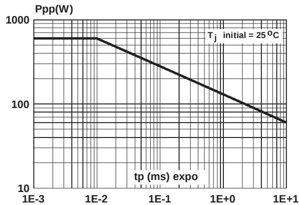
Fig. 1 : Typical peak pulse power versus exponential pulse duration.
