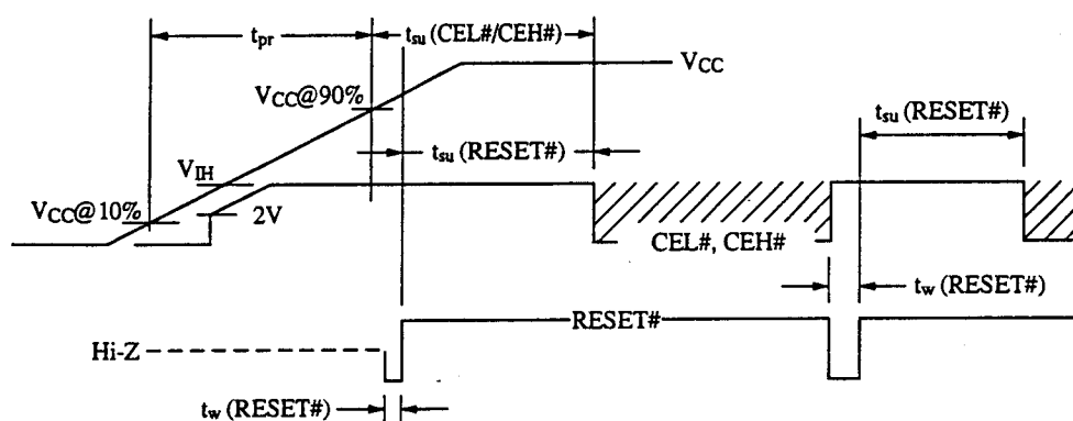
Power-Up Timing for Systems Supporting RESET#
