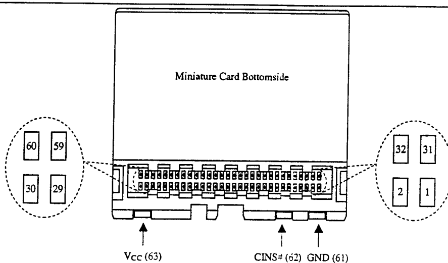
Figure 1. Card Interface Signal Assignment
