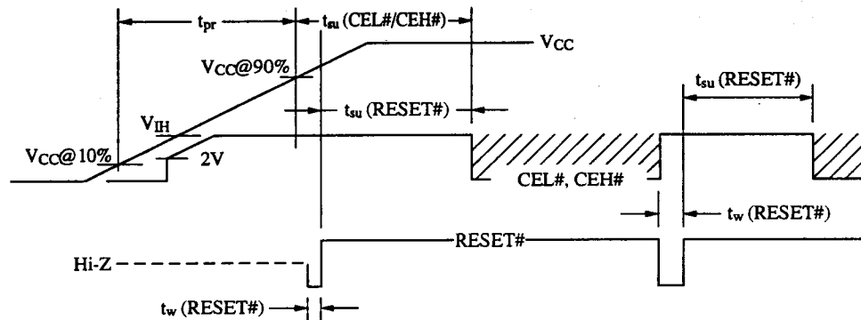
Power-Up Timing for Systems Supporting RESET#
