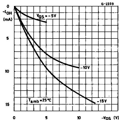
Minimum Output-p-channel Drain Characteristics.
