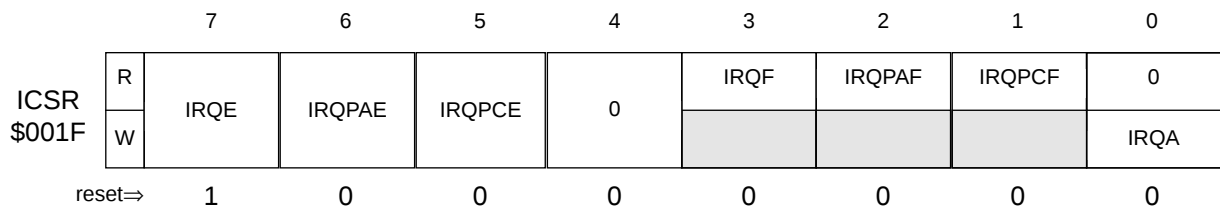
Figure 5-3: IRQ Status &amp; Control Register
