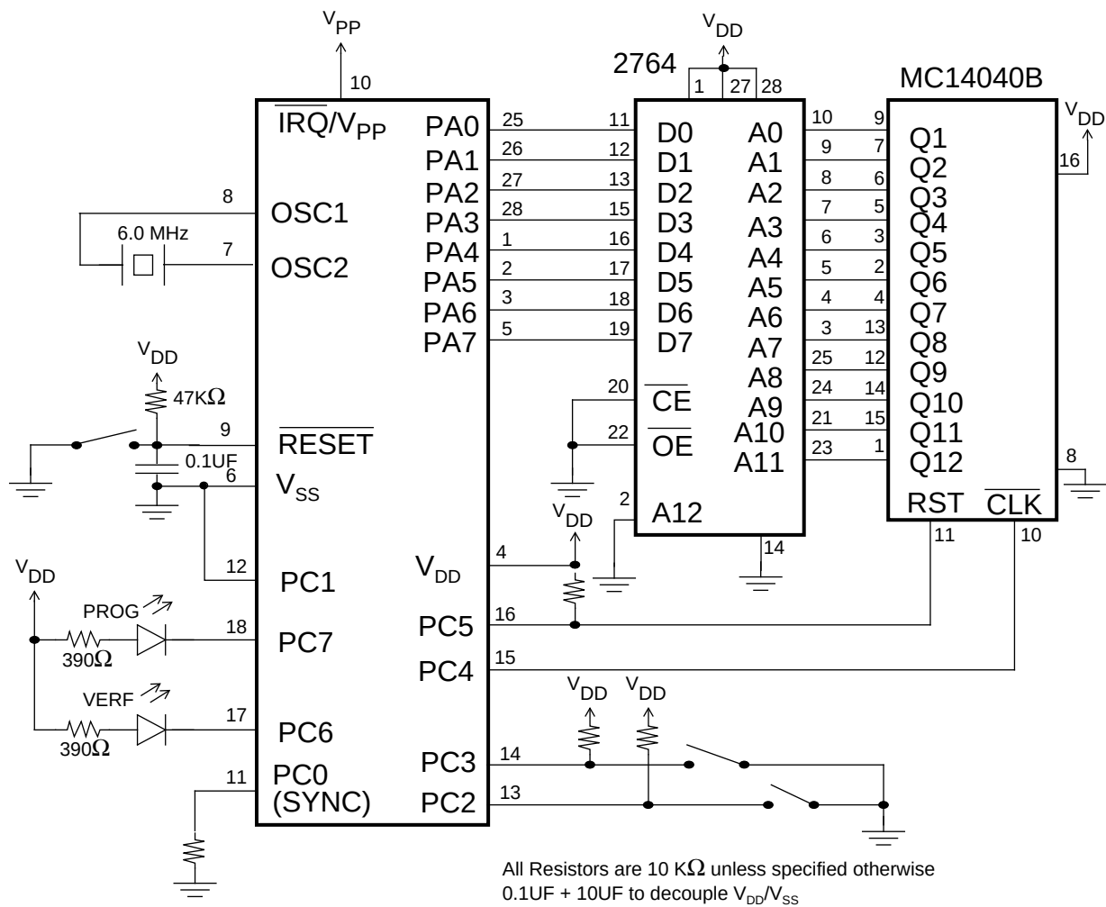
Figure 2-4: Programming Circuit
