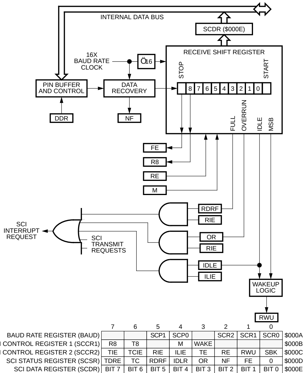
Figure 10-3: SCI Receiver
