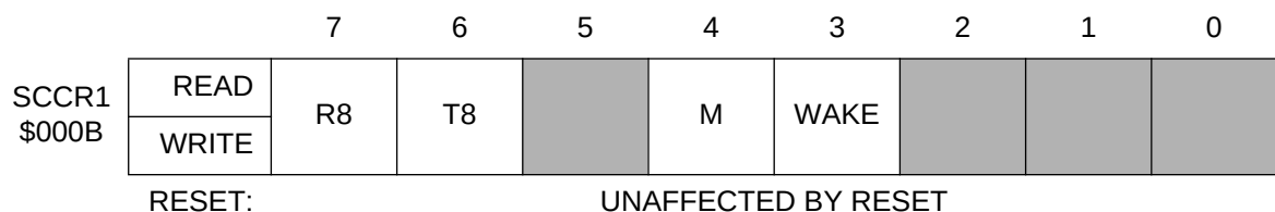
Figure 10-5: SCI Control Register 1 (SCCR1)
