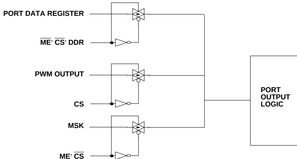
Figure 9-6: PWM Output MUX Logic
