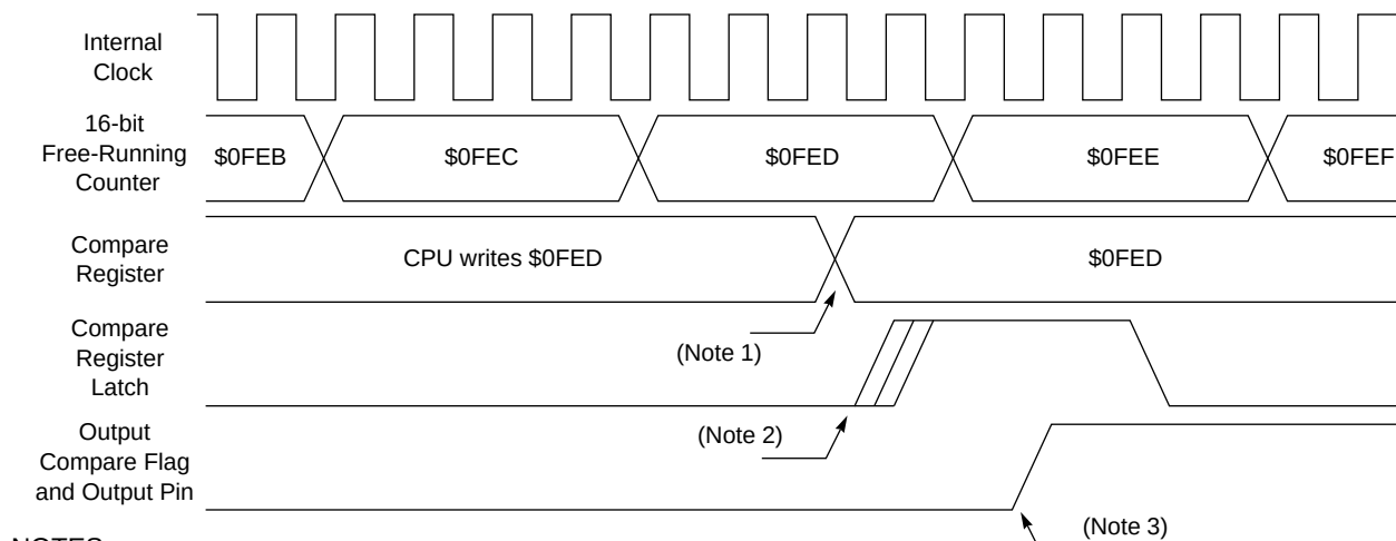
Figure 8-6: Output Compare Software Initialization Example
