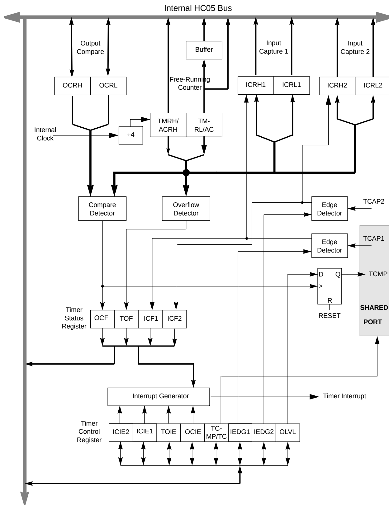
Figure 8-1: 16-Bit Timer Block Diagram
