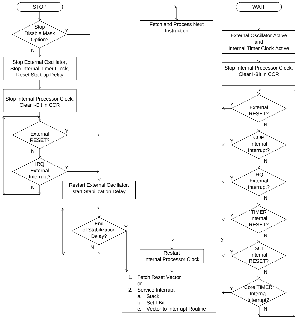
Figure 2-7: STOP/WAIT Flowcharts
