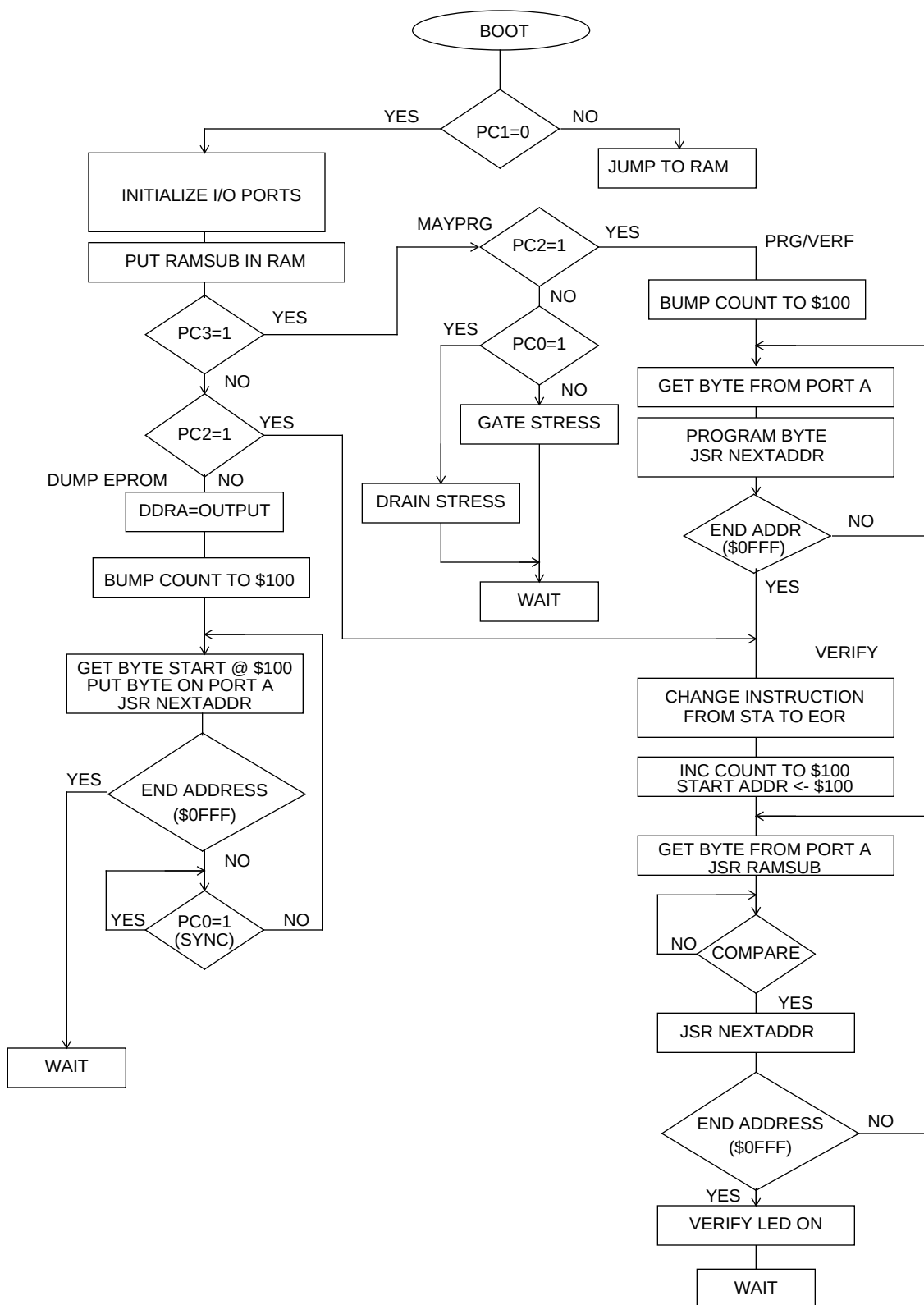
Figure 2-3: Bootloader Flowchart
