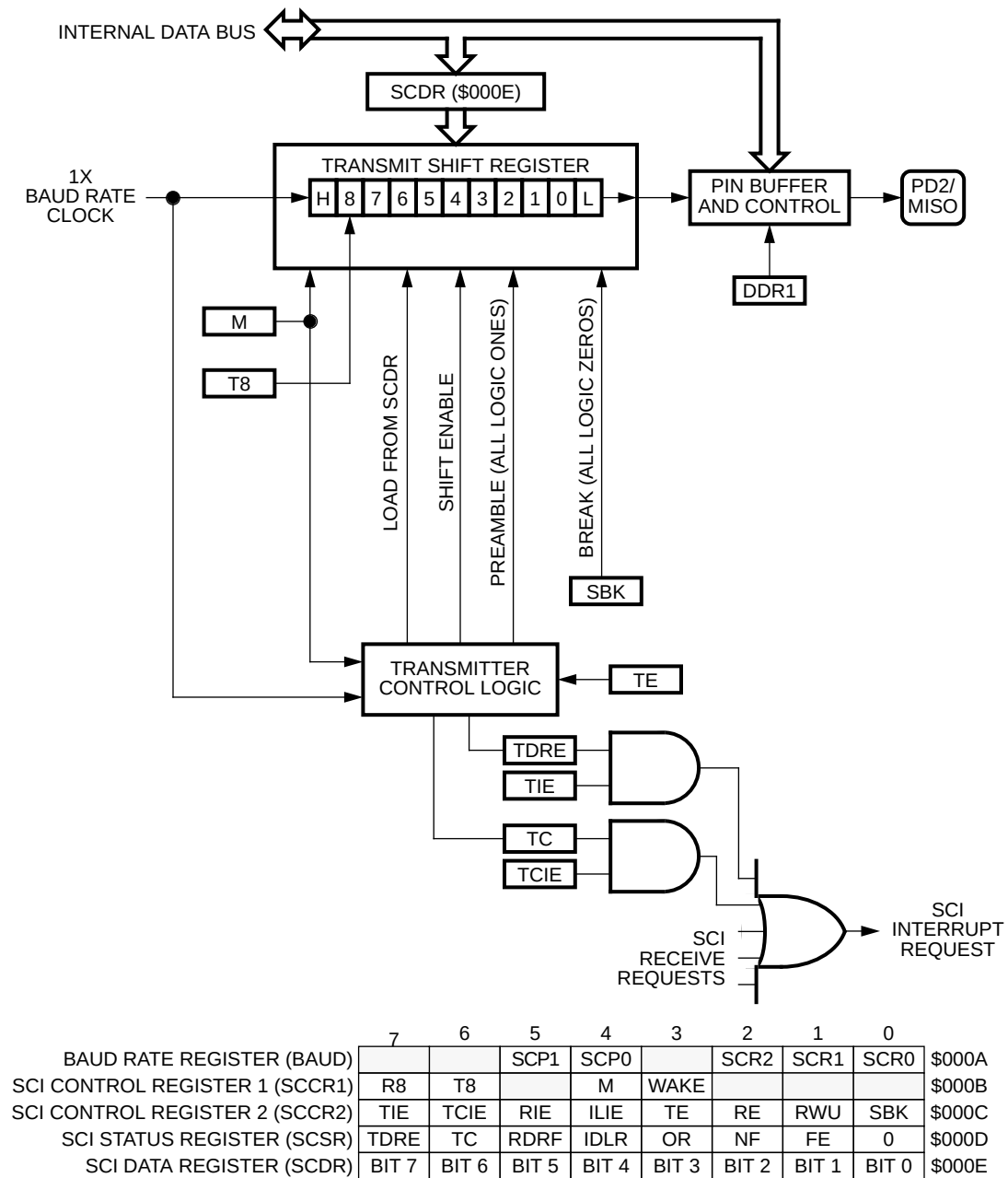
Figure 10-2: SCI Transmitter
