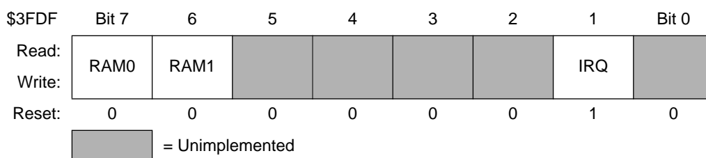
Figure 1-4. C9A Option Register
