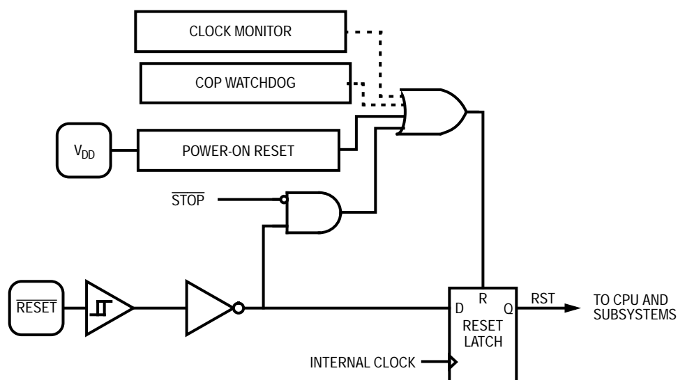
Figure 5-1. Reset Sources
