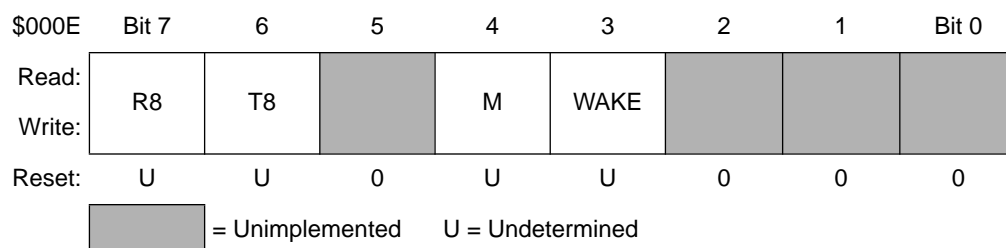
Figure 9-9. SCI Control Register 1 (SCCR1)
