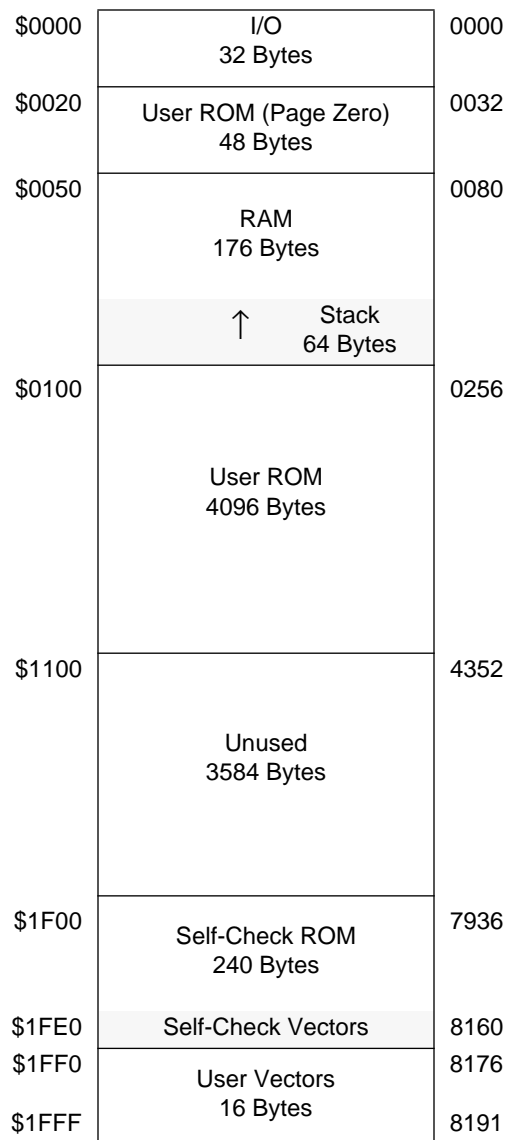
Figure 2-1. Memory Map
