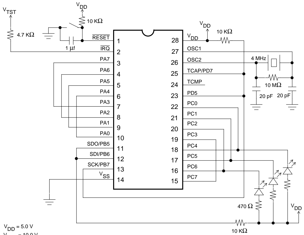
Figure 10-1. Self-Check Circuit
