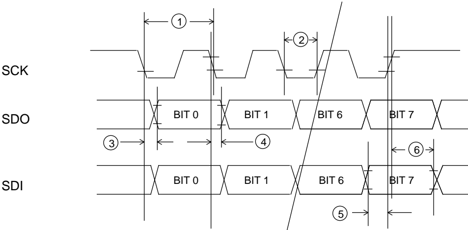
Figure 12-1. SIOP Timing Diagram
