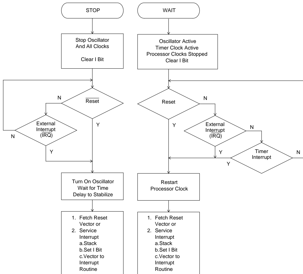
Figure 4-6: STOP/WAIT Flowcharts
