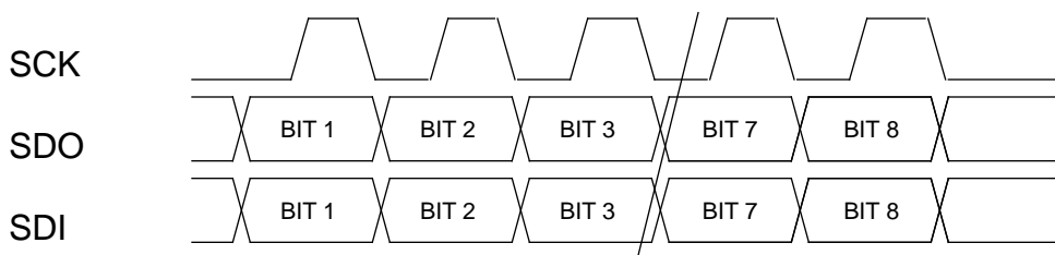
Figure 7-3: Serial I/O Port Timing (CPOL=0)
