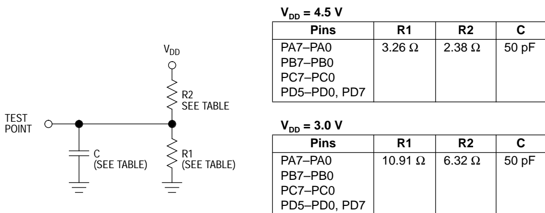
Figure 13-1. Test Load
