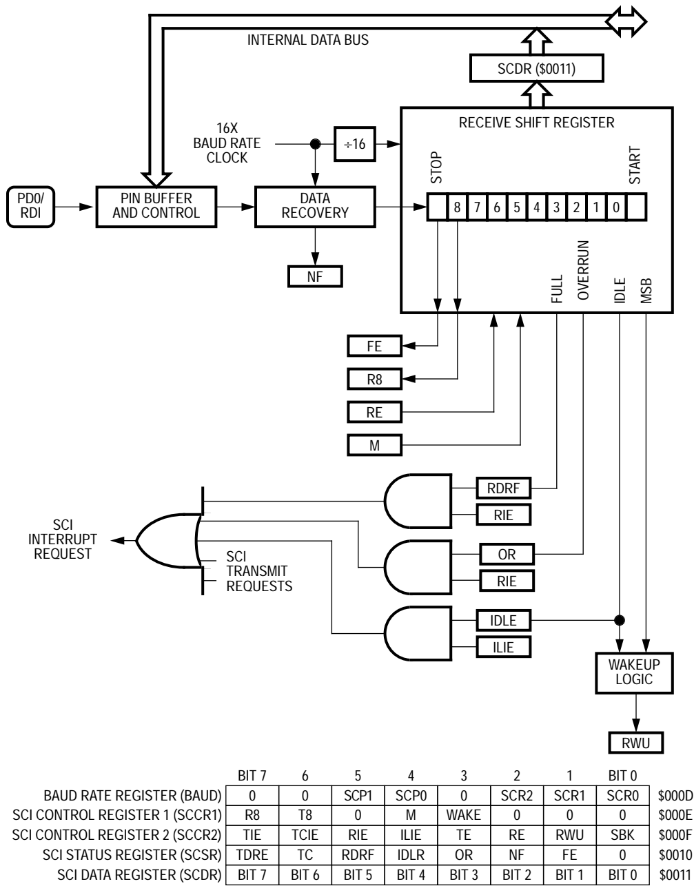
Figure 9-3. SCI Receiver
