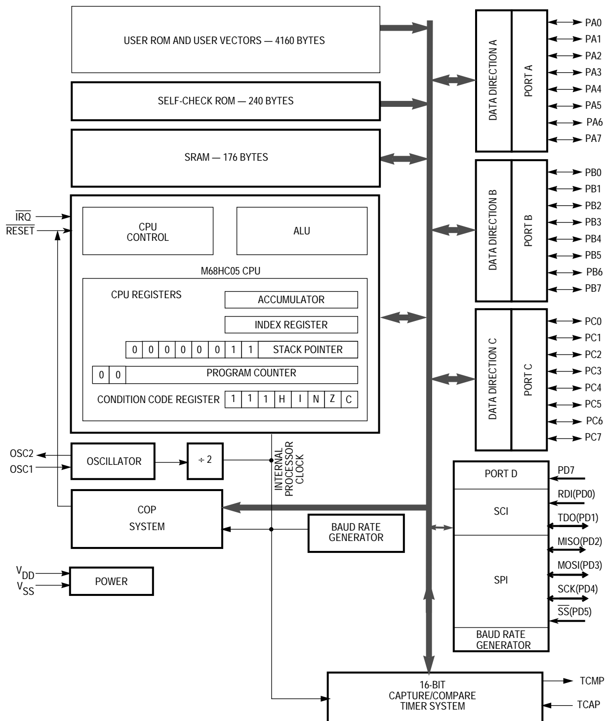
Figure 1-1. Block Diagram
