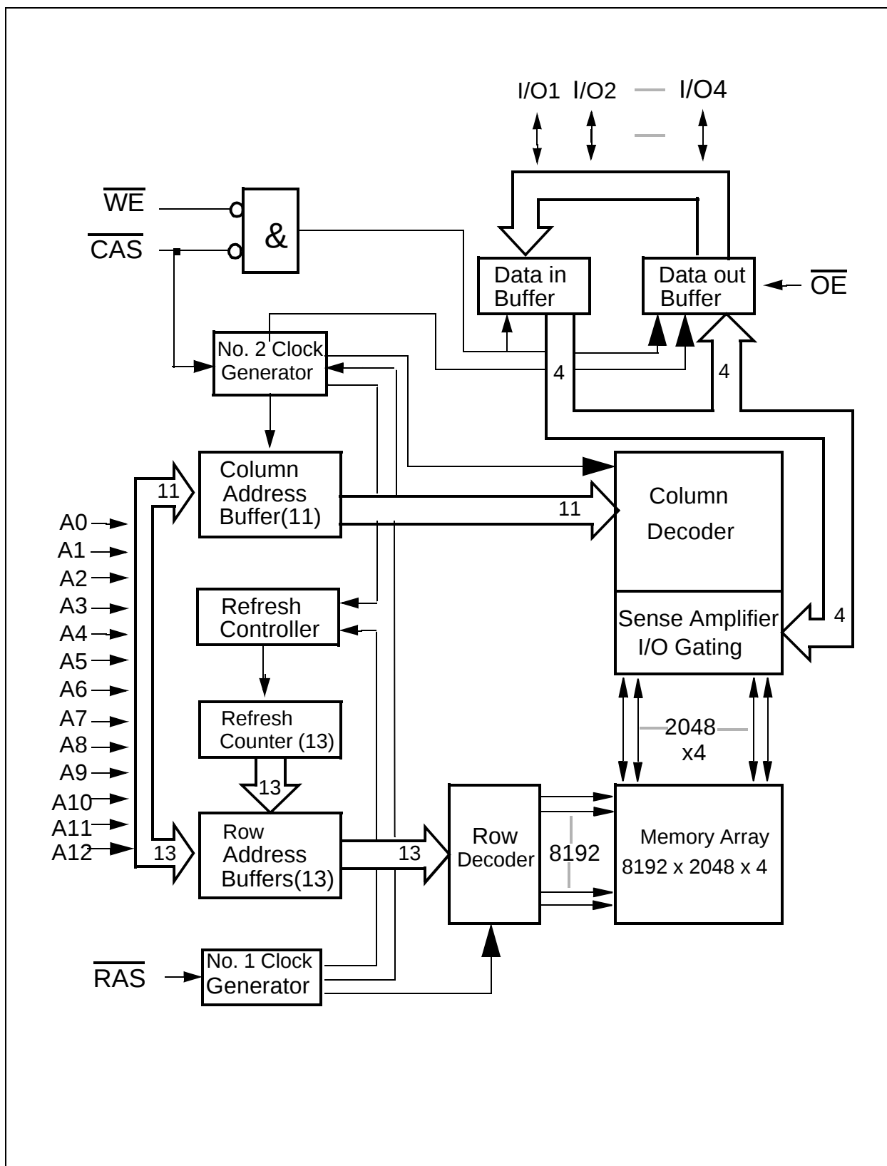
Block Diagram for HYB 3165405BJ/BT(L)
