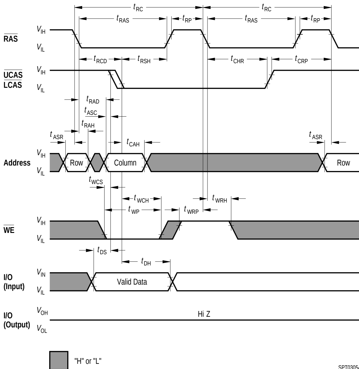
Hidden Refresh Cycle (Early Write)
