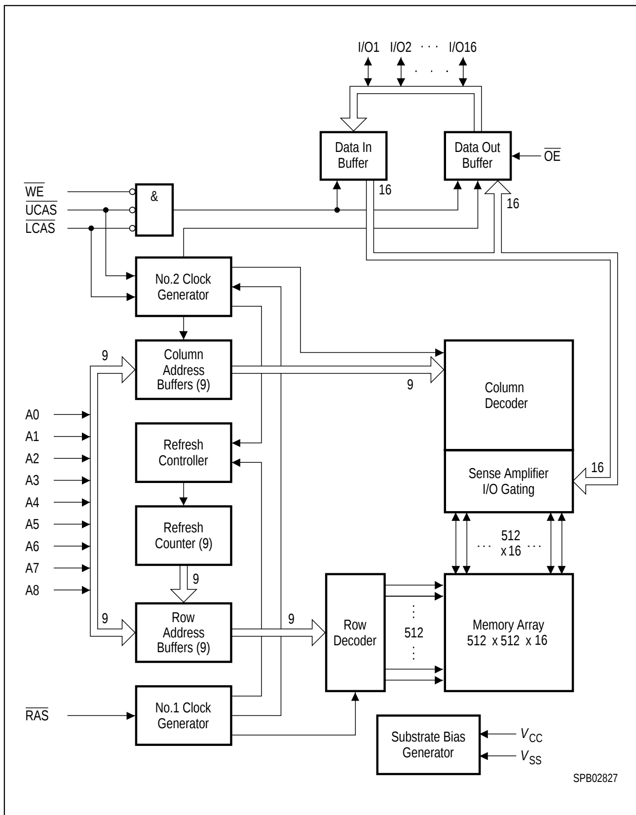
Block Diagram
