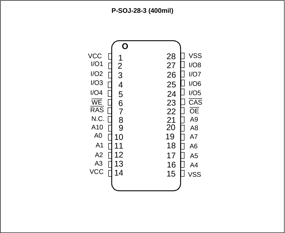
Pin Configuration
