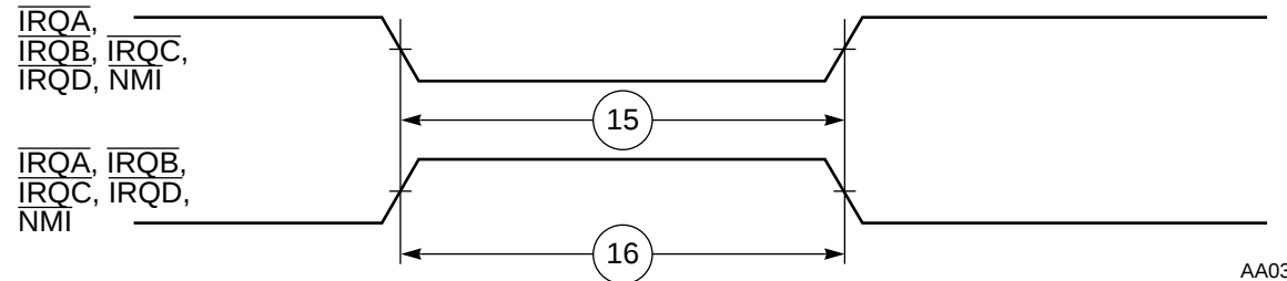
Figure 2-6 External Interrupt Timing (Negative Edge-Triggered)
