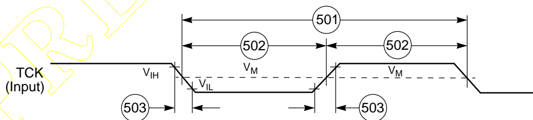
Figure 2-39 Test Clock Input Timing Diagram
