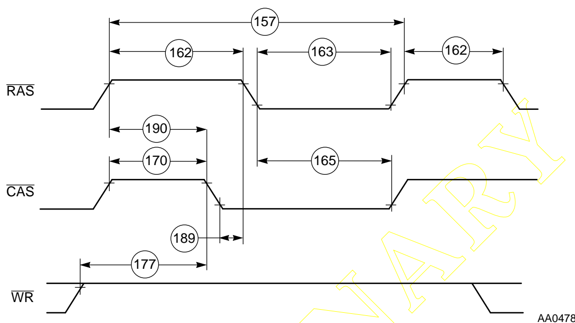
Figure 2-20 DRAM Refresh Access
