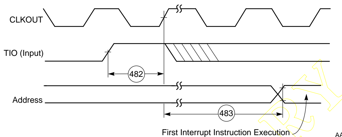
Figure 2-42 Timer Interrupt Generation
