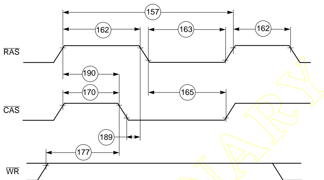
Figure 2-20 DRAM Refresh Access
