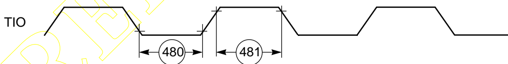
Figure 2-41 TIO Timer Event Input Restrictions
