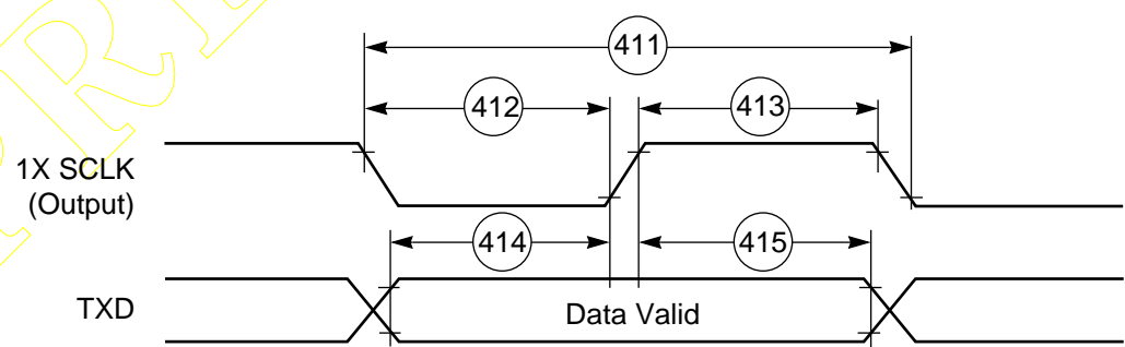
Figure 2-38 SCI Asynchronous Mode Timing
