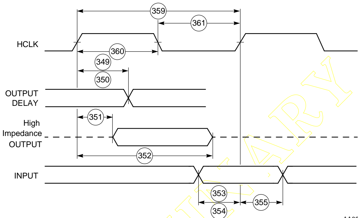
Figure 2-35 PCI Timing
