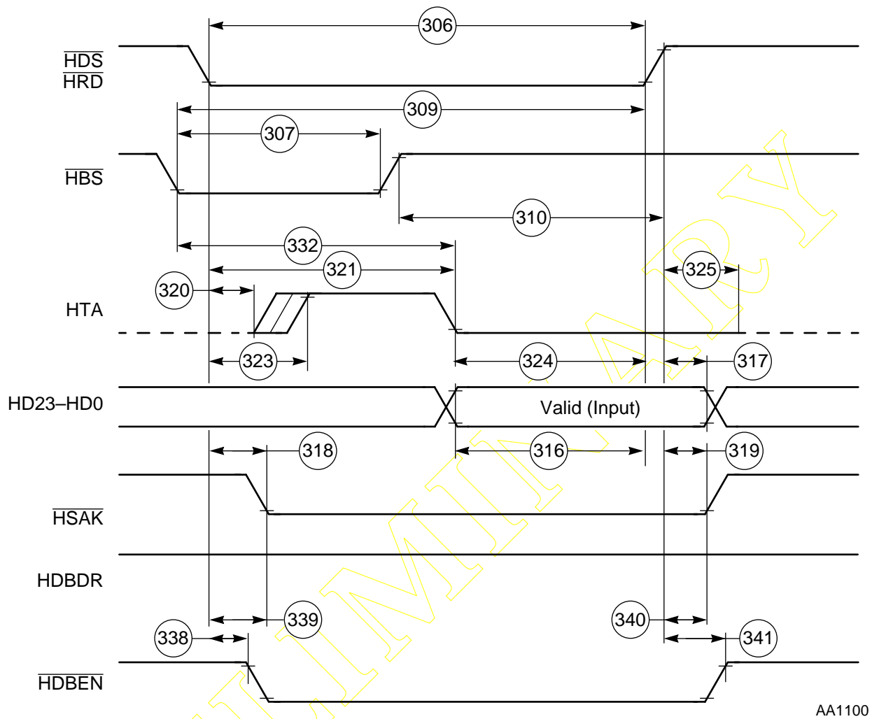
Figure 2-32 Write Timing
