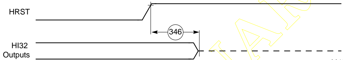
Figure 2-30 HRST Timing
