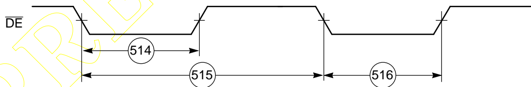
Figure 2-49 OnCE—Debug Request
