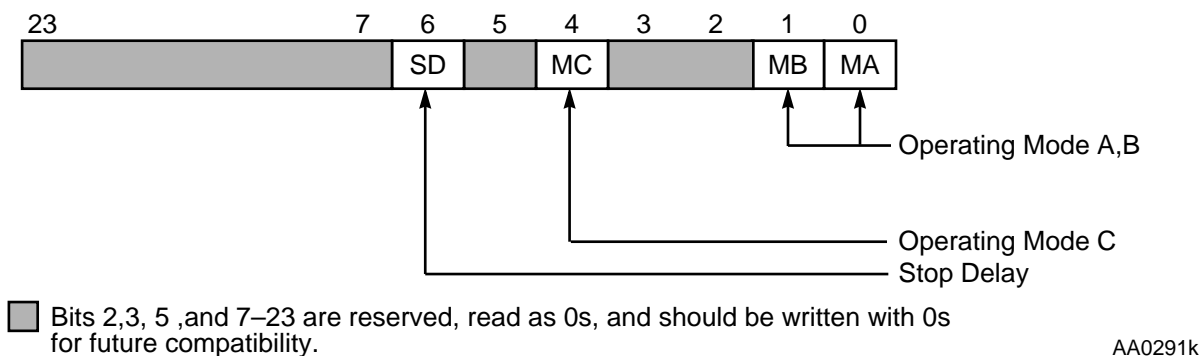
Figure 3-3 Operating Mode Register (OMR)
