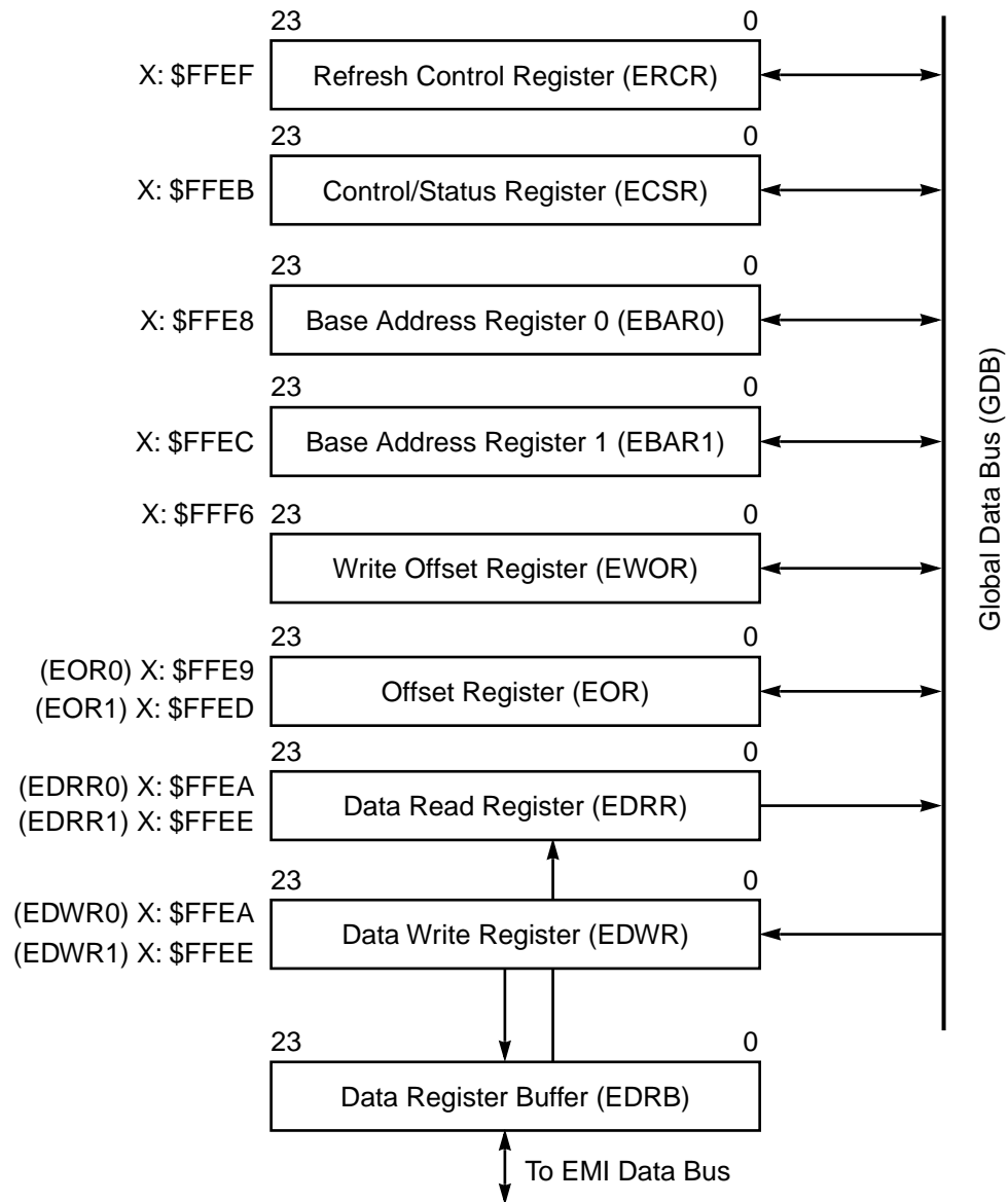
Figure 4-1 EMI Registers
