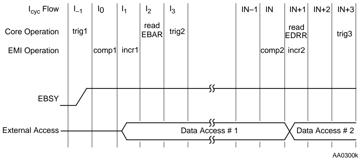
Figure 4-8 EMI Pipeline
