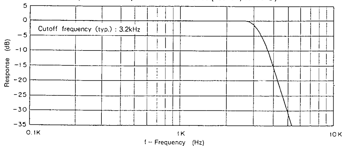
Splatter filter amplitude characteristics ( V_{DD}=5V , T_a=25^\circ C )
