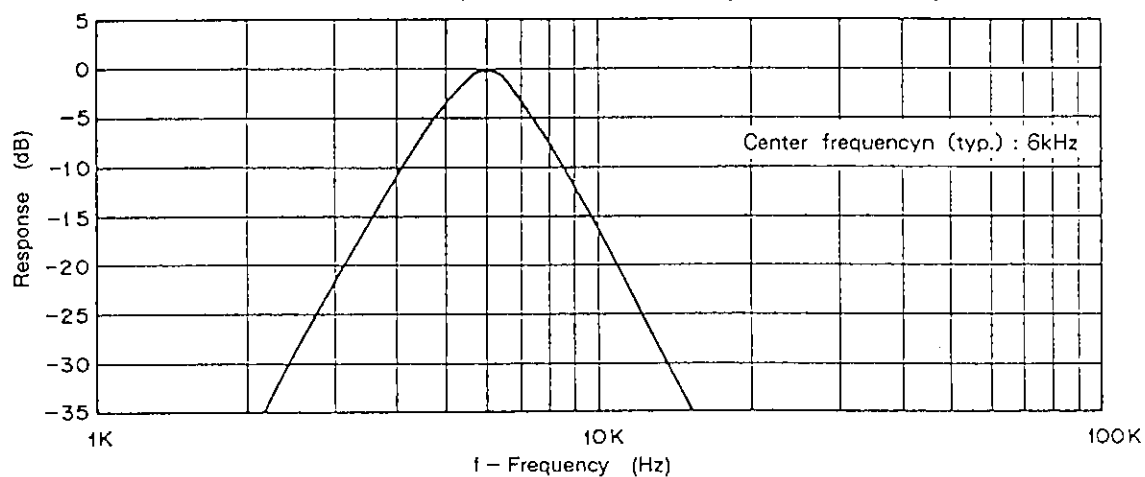
Received SAT BPF amplitude characteristics ( V_{DD}=5V , T_a=25^\circ C )
