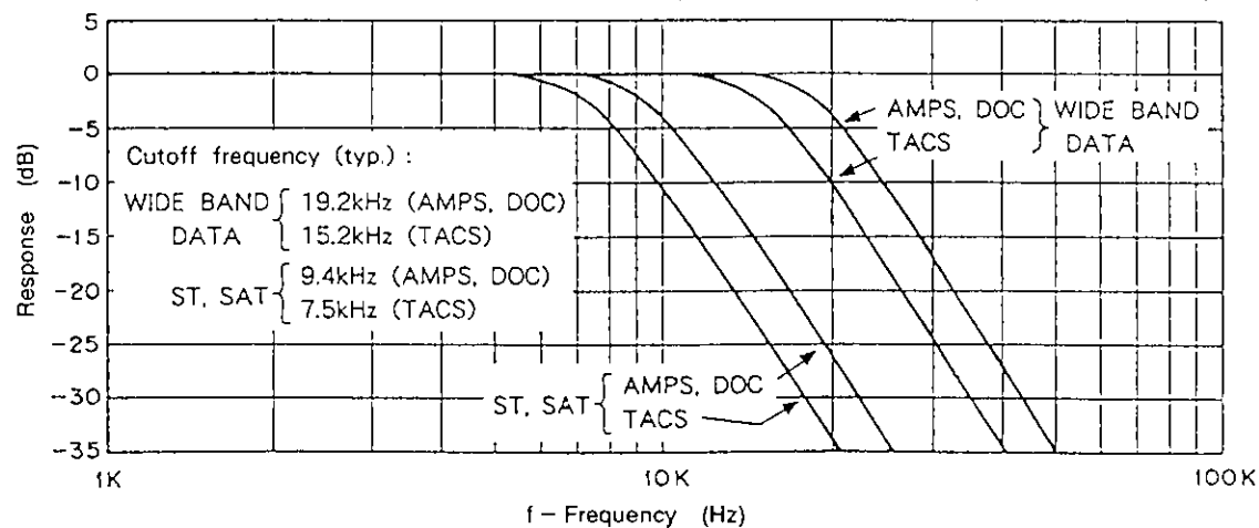
Transmitted WIDE BAND DATA, ST, SAT LPF amplitude characteristics ( V_{DD}=5V , T_a=25^\circ C )
