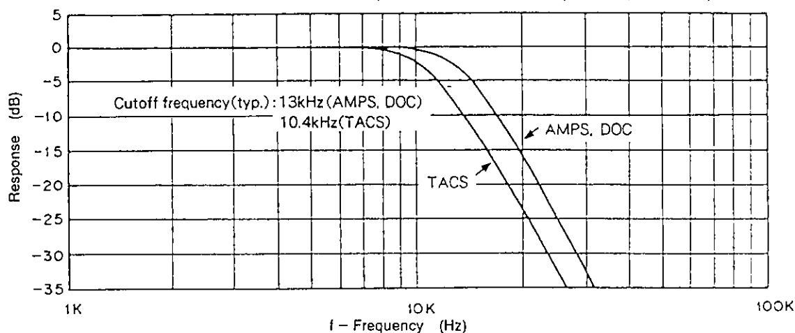
Received WIDE BAND DATA LPF amplitude characteristics ( V_{DD}=5V , T_a=25^\circ C )
