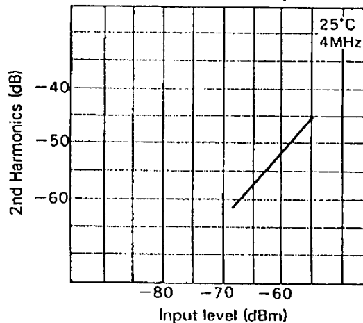
2nd Harmonics vs. Input level
