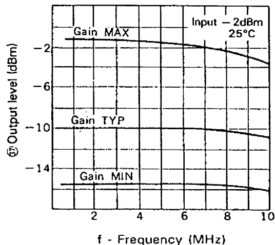
Output level vs. Frequency
