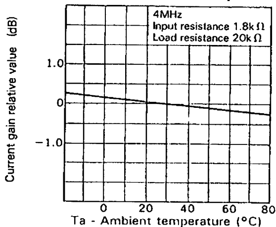
Current gain vs. Ambient temperature
