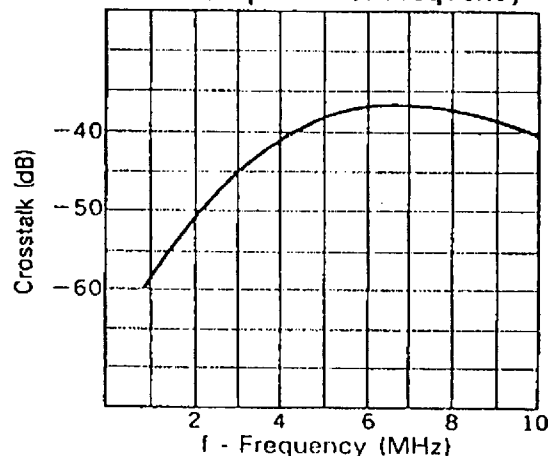
CH-1 → CH-2 crosstalk with PB RF output 2 vs. Frequency
