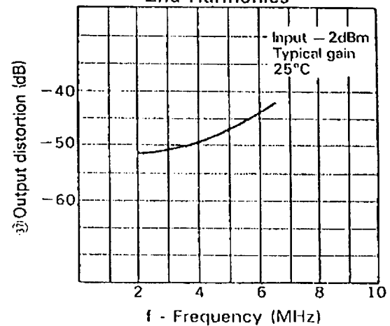
2nd Harmonics
