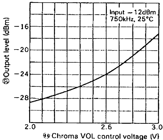
Output level vs. Chroma VOL control voltage
