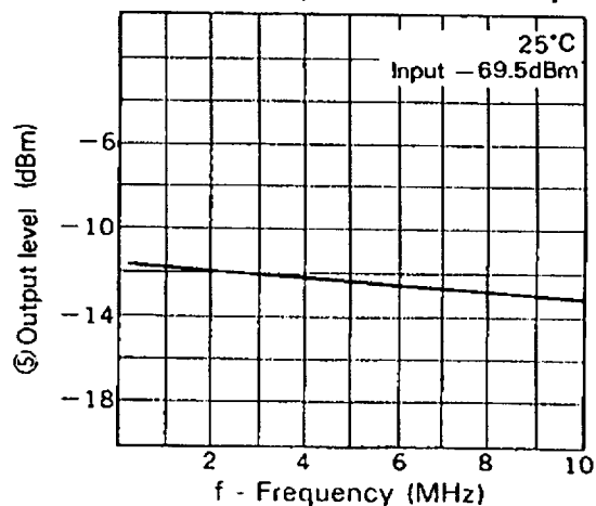
RF output 2 output level vs. Frequency
