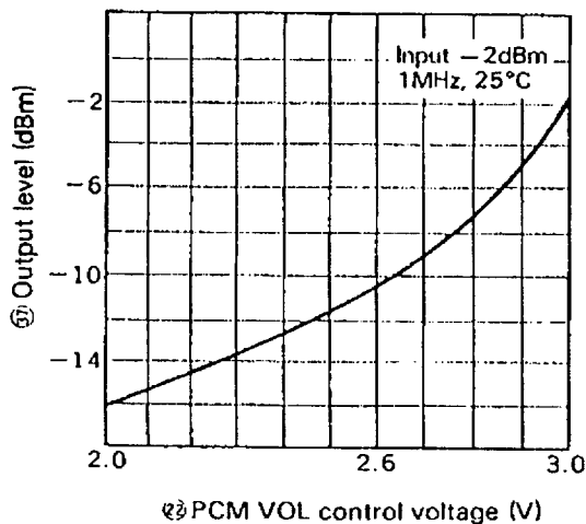
Output level vs. PCM VOL control voltage
