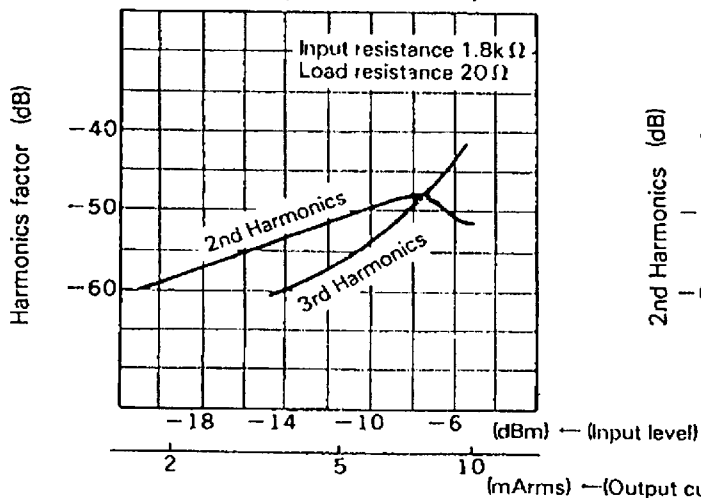
Distortion factor vs. Input level, Output current
