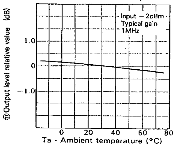
ATF VOL + SW Typical Performance Curves
