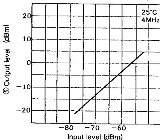
RF output 2 output level vs. PB input level
