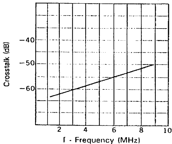
REC PCM VOL + SW crosstalk vs. Frequency
