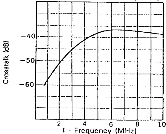
CH-2 → CH-1 crosstalk with PB RF output 2 vs. Frequency
