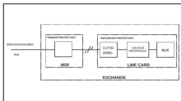
Fig.1 : Subscriber line protection topology
