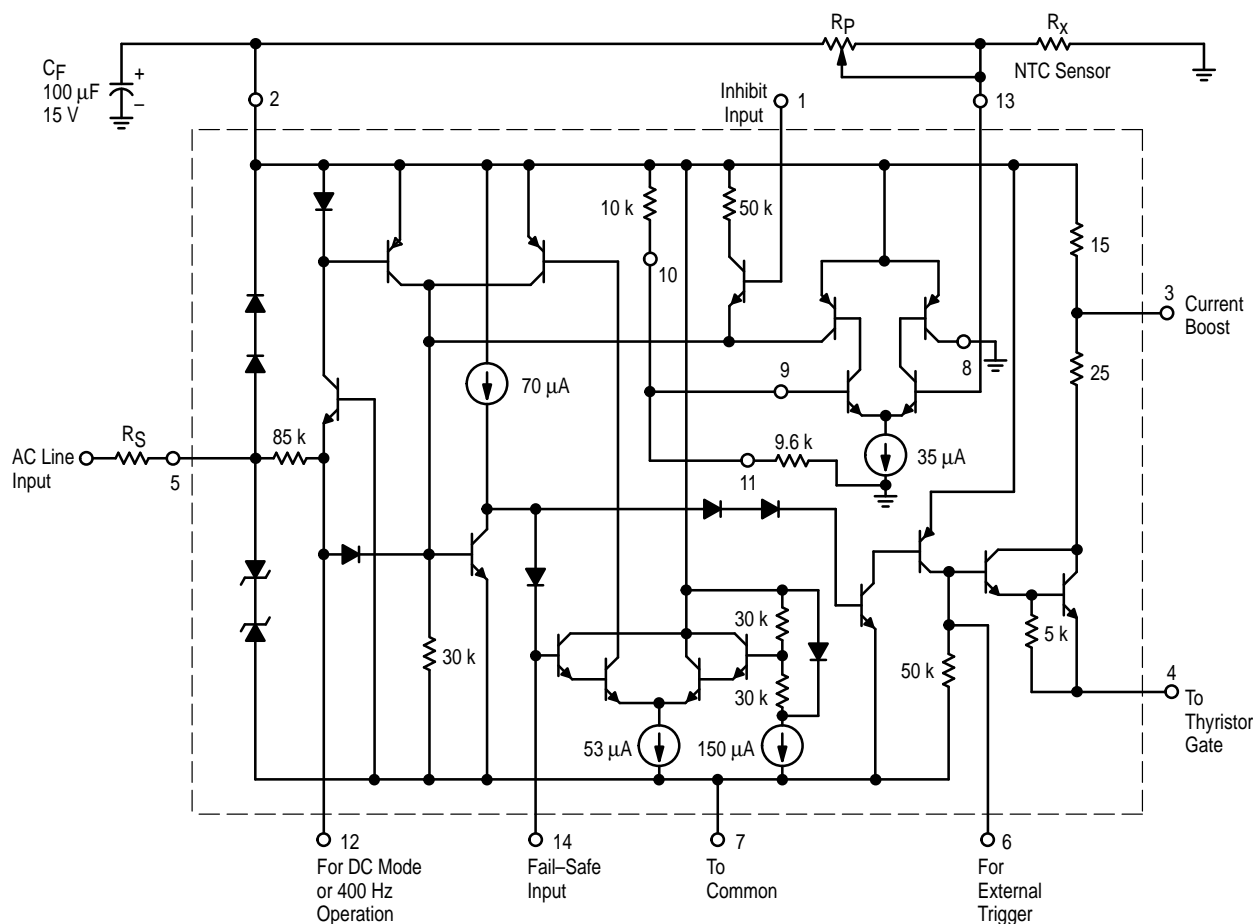
Figure 14. Circuit Schematic
