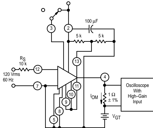
Figure 4. Peak Output Current (Pulsed) with External Power Supply
