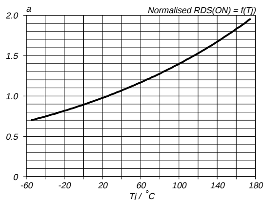
Fig. 9. Normalised drain-source on-state resistance. a = R_{DS(ON)} / R_{DS(ON)25^\circ \text{C}} = f(T_j) ; I_D = 29 \text{ A} ; V_{GS} = 10 \text{ V}
