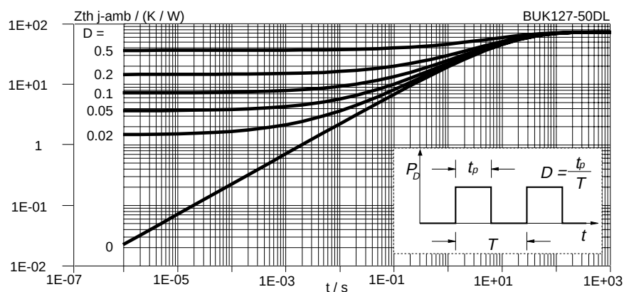
Fig.19. Transient thermal impedance, mounted on SOT223 PCB.
