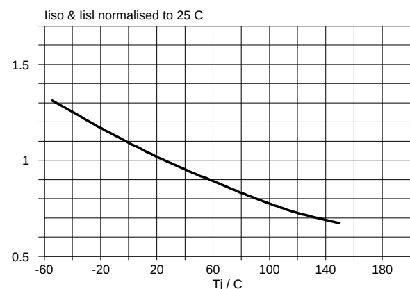
Fig.21. Normalised input currents (normal & latched). I_{ISO}/I_{ISO\ 25^\circ\text{C}} & I_{ISL}/I_{ISL\ 25^\circ\text{C}} = f(T_j) ; V_{IS} = 5\text{ V}
