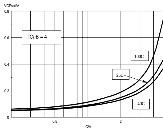
Fig. 12. Collector-Emitter saturation voltage. Solid lines = typ values, V_{CEsat} = f(I_C)
