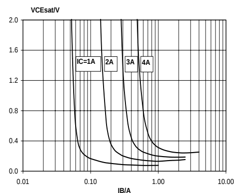
Fig. 10. Collector-Emitter saturation voltage. Solid lines = typ values, V_{CEsat} = f(I_B) ; T_J = 25^\circ C
