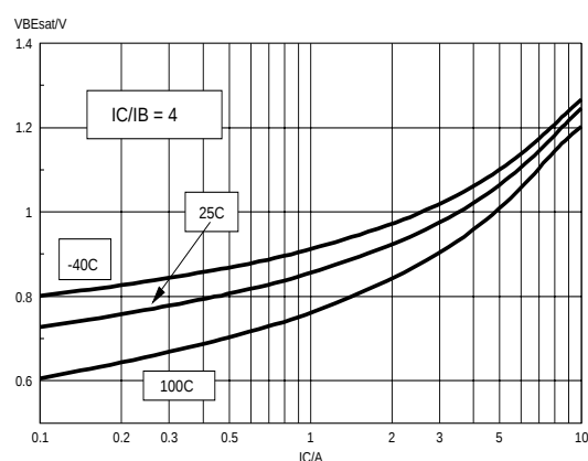
Fig. 11. Base-Emitter saturation voltage. Solid lines = typ values, V_{BEsat} = f(I_C)
