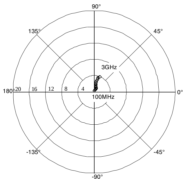
Fig.10 Common emitter reverse transmission coefficient ( S_{12} ); typical values.
