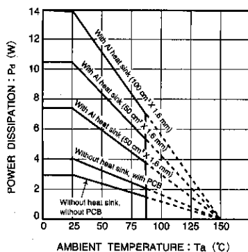
Fig.1 Thermal derating curves
