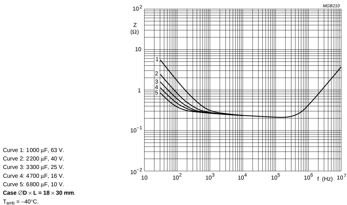
Fig.18 Typical impedance as a function of frequency.
