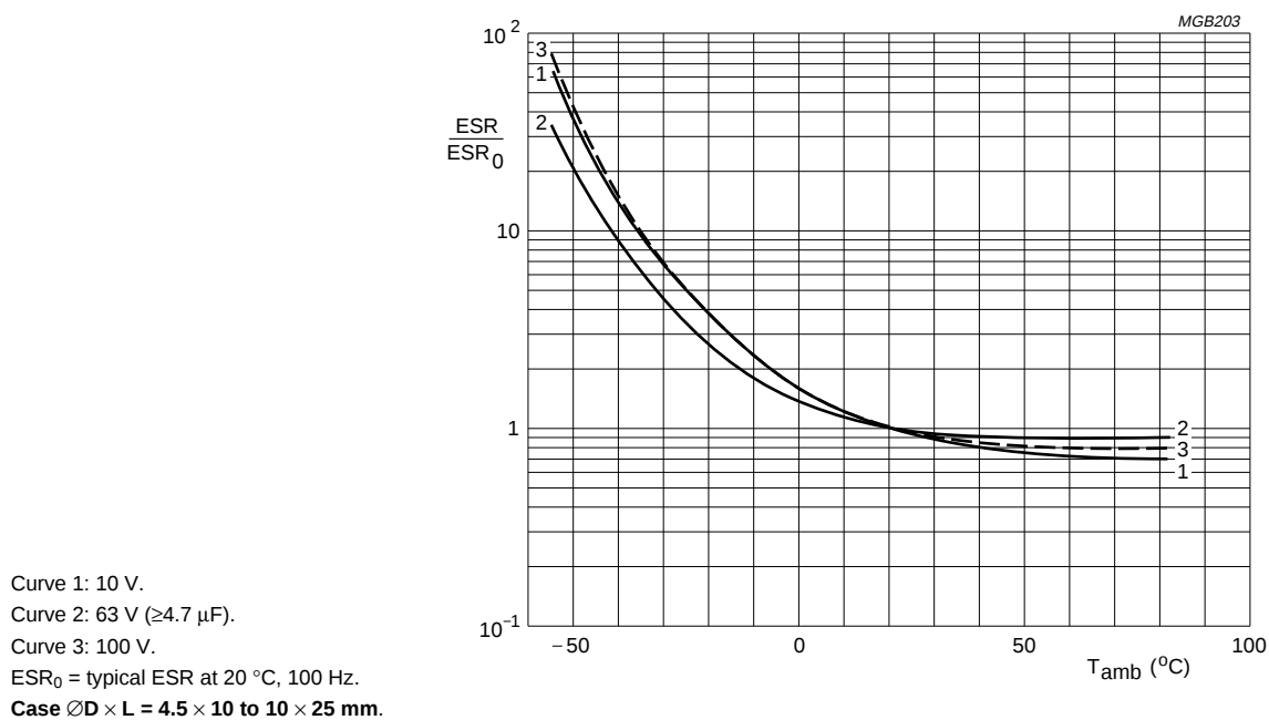
Fig.9 Typical multiplier of ESR as a function of ambient temperature.
