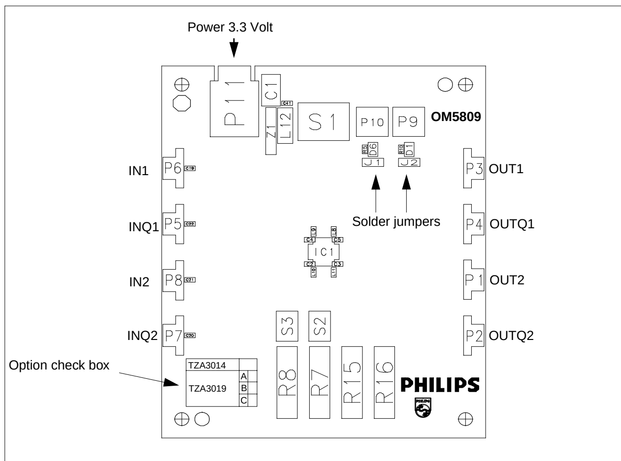
Fig.2 OM5809 demoboard
