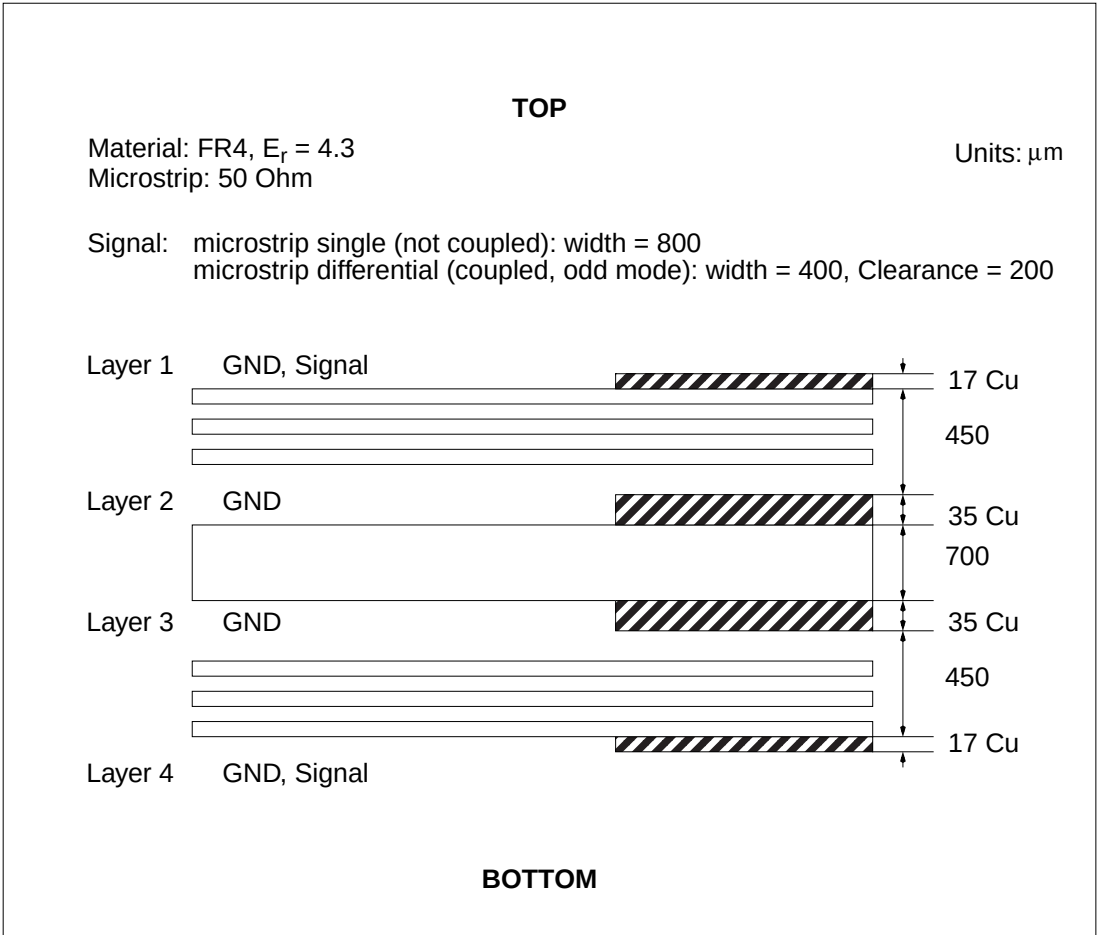
Fig.3 Cross section of multi layer PCB
