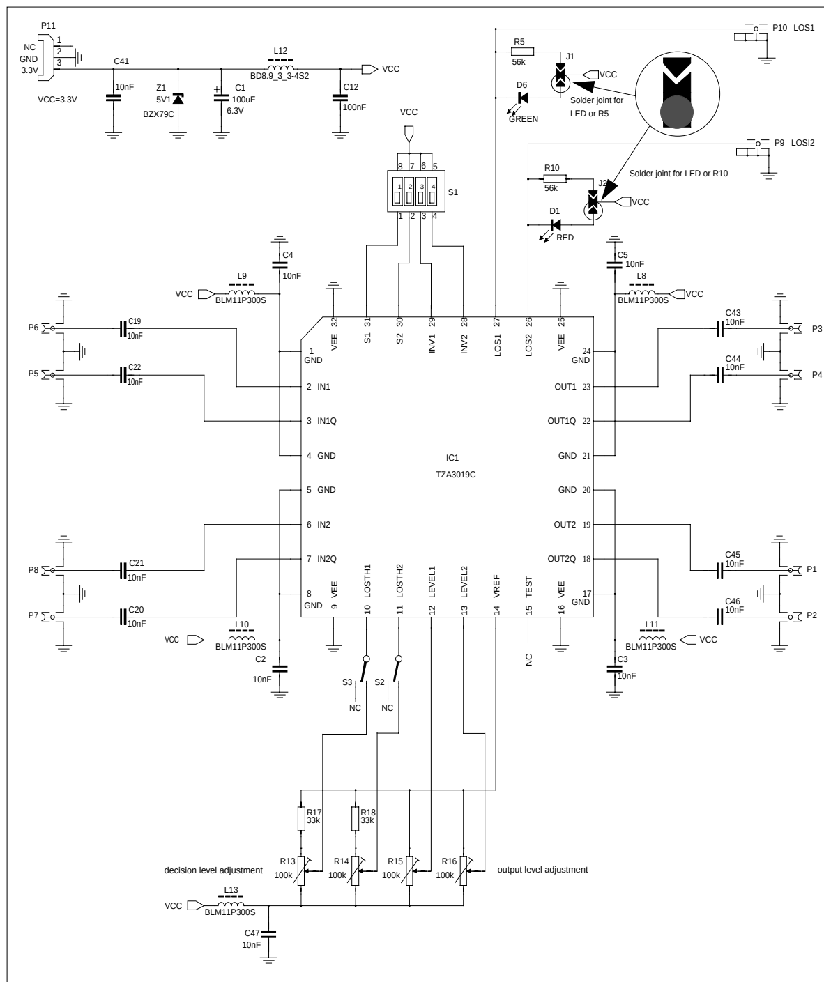
Fig.8 Schematic of OM5809 demoboard with TZA3019C
