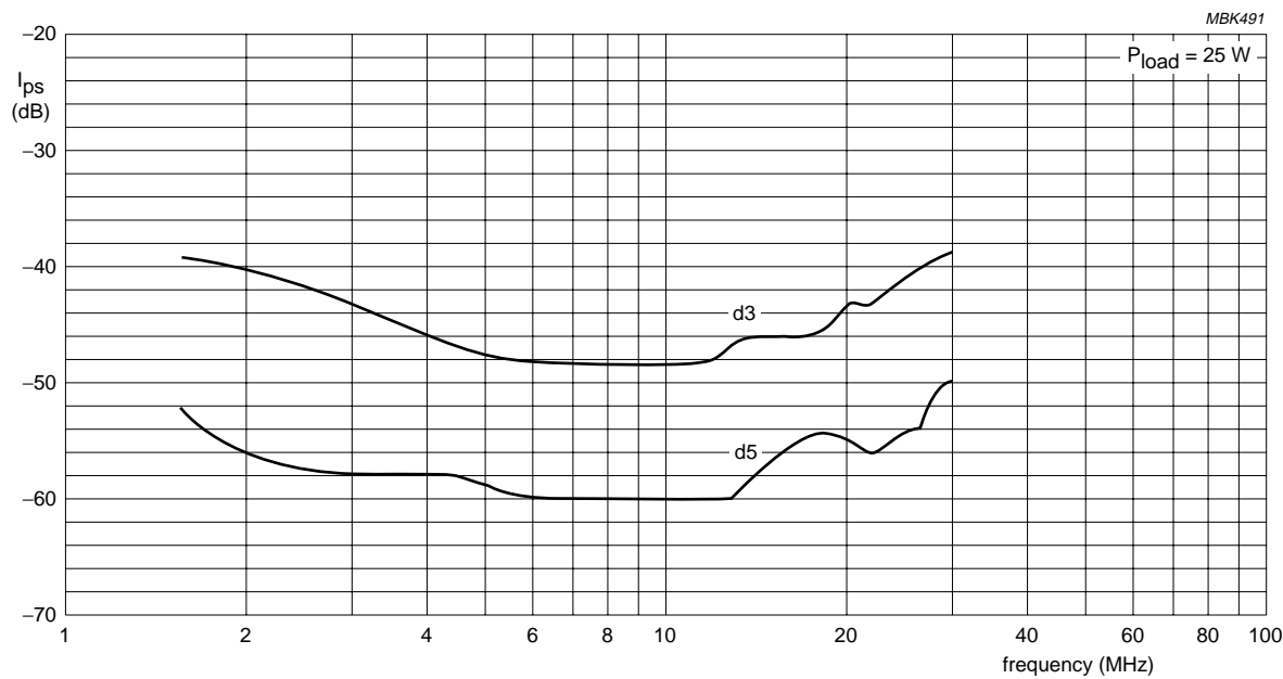
Fig.11 BLW50F linear amplifier-intermodulation products versus frequency.
