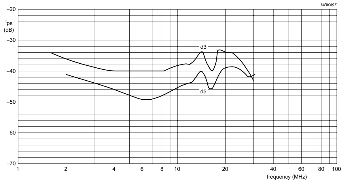
Fig.17 Intermodulation performance (50 V, 200 W PEP).
