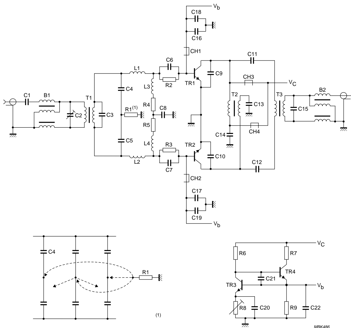
Fig.1 Circuit diagram of BLW96 power amplifier for 1.6 – 30 MHz, 400 W PEP, see Table 2 for parts list.
