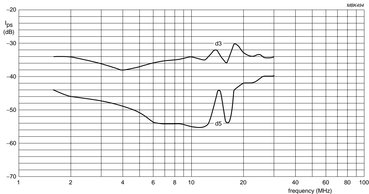
Fig.20 Intermodulation performance (45 V, 300 W PEP).
