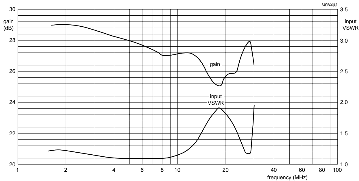
Fig.16 Amplifier gain and VSWR.
