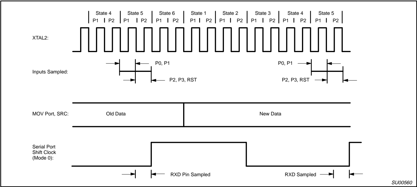
Figure 34. Port Operation
