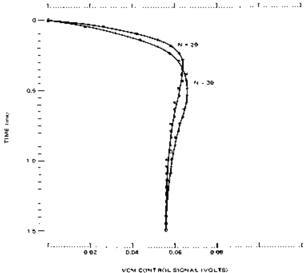
Figure 15. VCM Control Signal Transient
