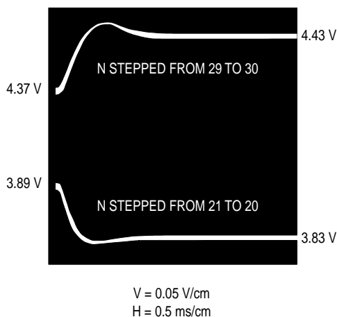
Figure 14. VCM Control Voltage (Frequency) Transient
