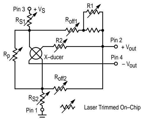
Figure 1. Pressure Sensor MPX2000 Series
