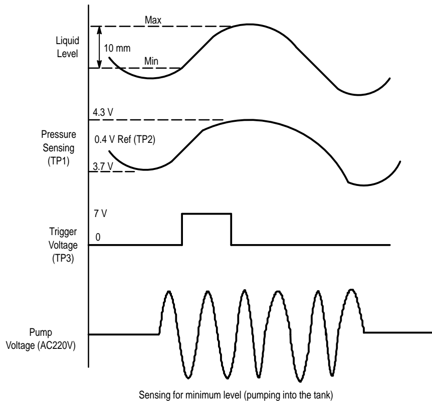
Figure 5. Functional Diagram
