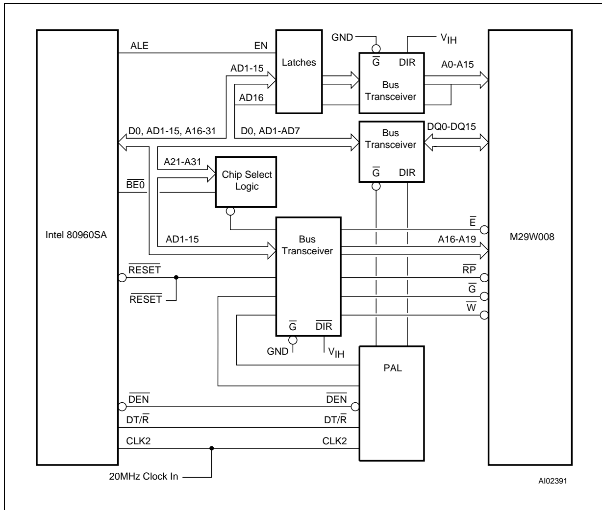
Figure 2. Connection of the M29W008 to the 80960SA
