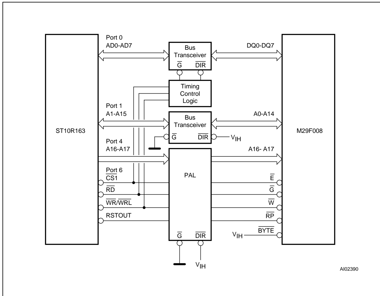
Figure 1. Connection of the M29F008 to the ST10R163
