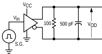
Figure 3. Differential Mode Rise/Fall Time and Data Propagation Delay
