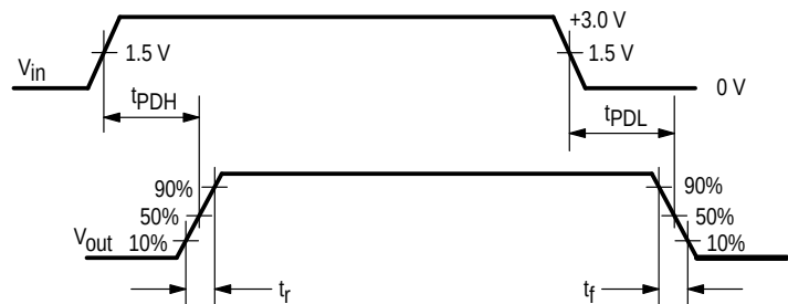
Figure 3. Differential Mode Rise/Fall Time and Data Propagation Delay
