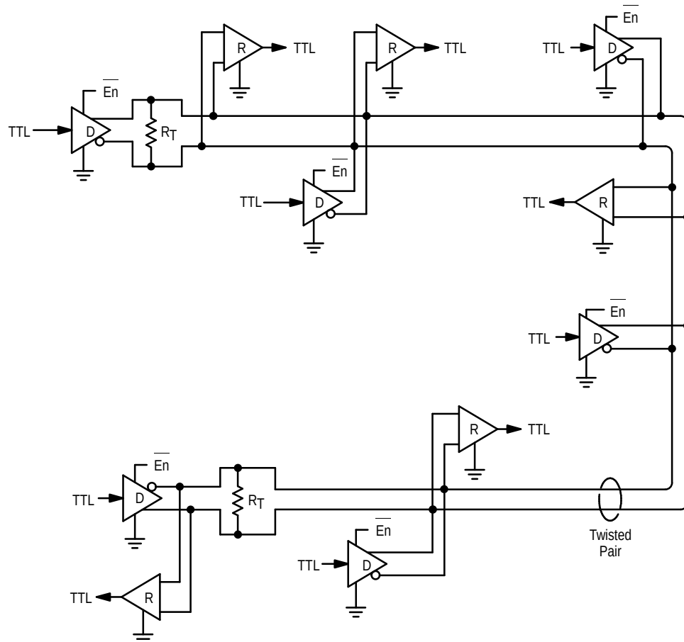
Figure 17. EIA-422-A Example
