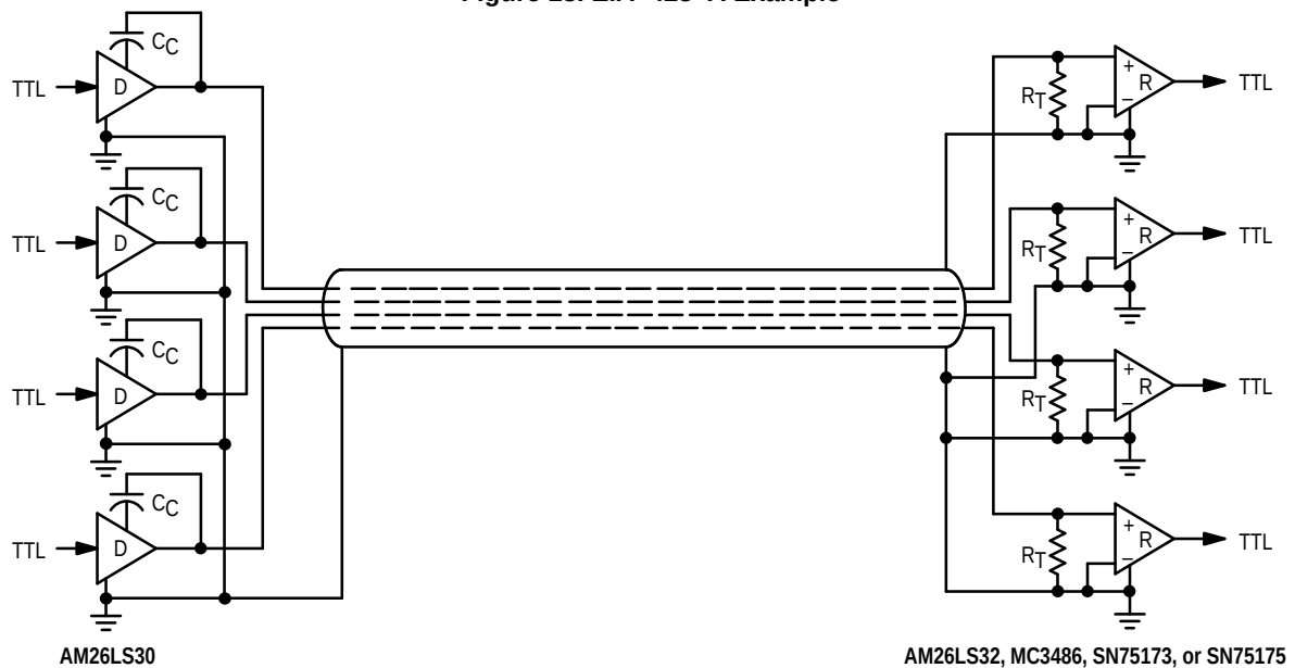
Figure 18. EIA-423-A Example
