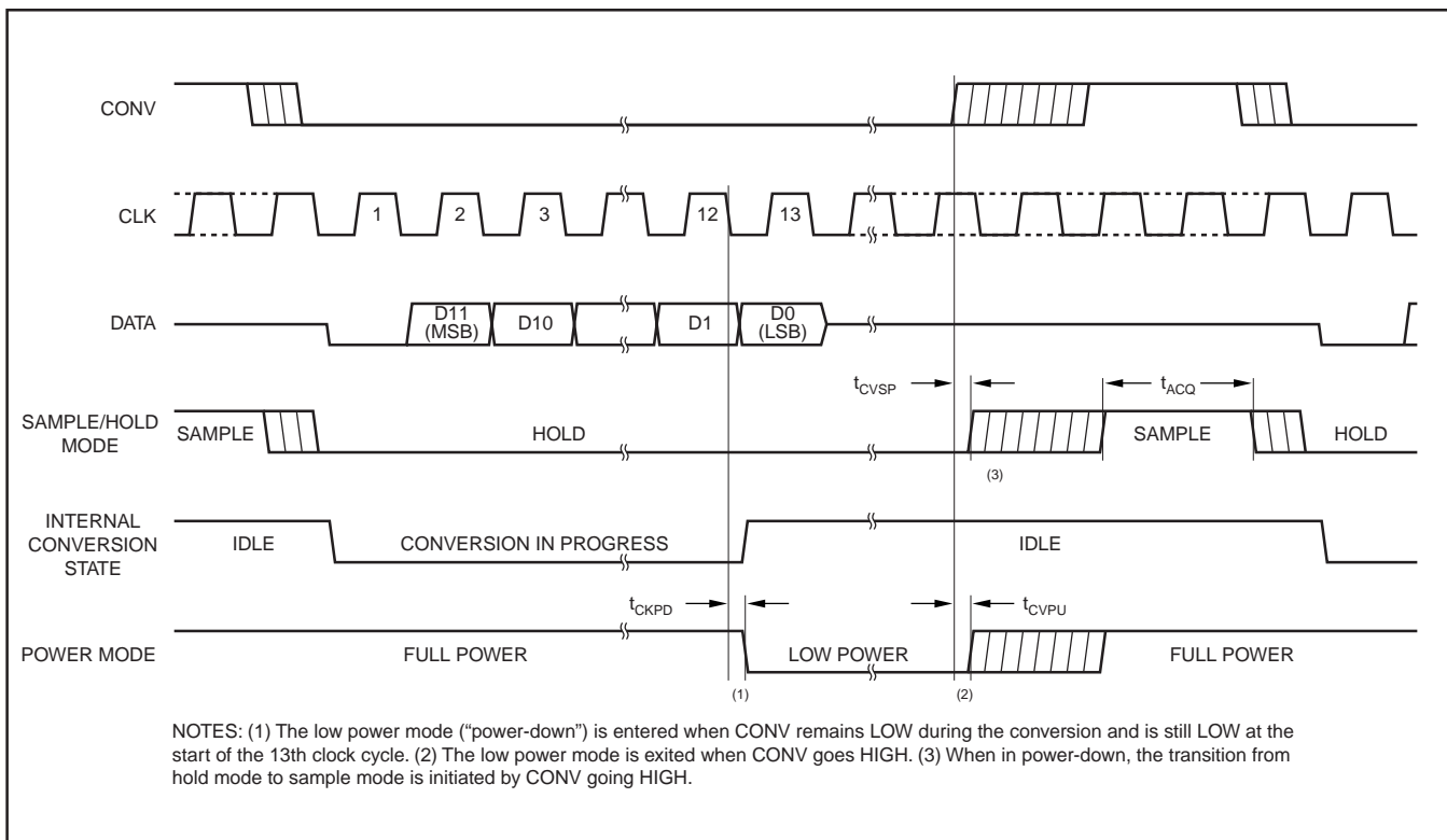
FIGURE 4. Power-Down Timing.
