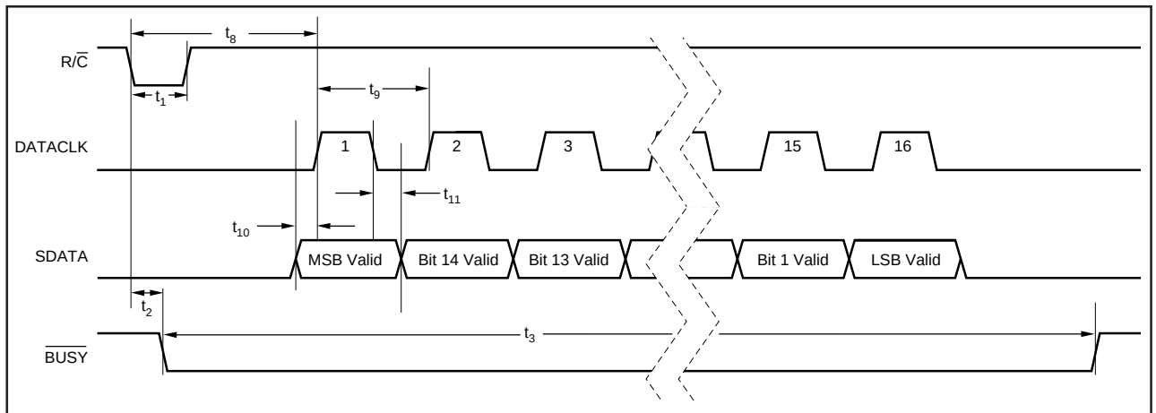
FIGURE 2. Serial Data Timing Using Internal Clock. ( \overline{\text{CS}} , \text{EXT}/\overline{\text{INT}} and TAG Tied LOW.)
