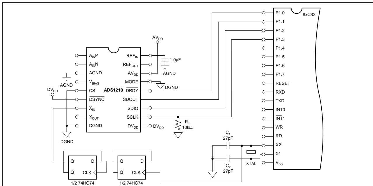
FIGURE 30. Four-Wire Interface with a 8xC32 Microprocessor.
