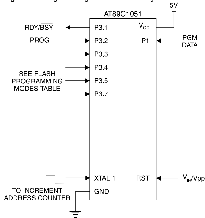
Figure 3. Programming the Flash Memory
