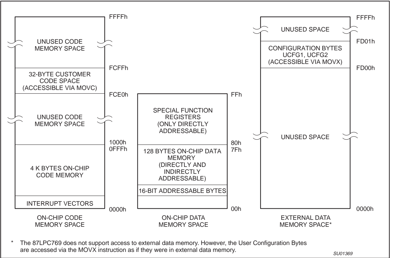
Figure 1. 87LPC769 Program and Data Memory Map
