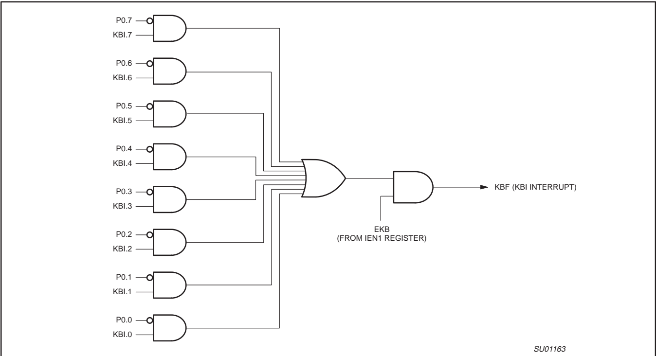
Figure 17. Keyboard Interrupt
