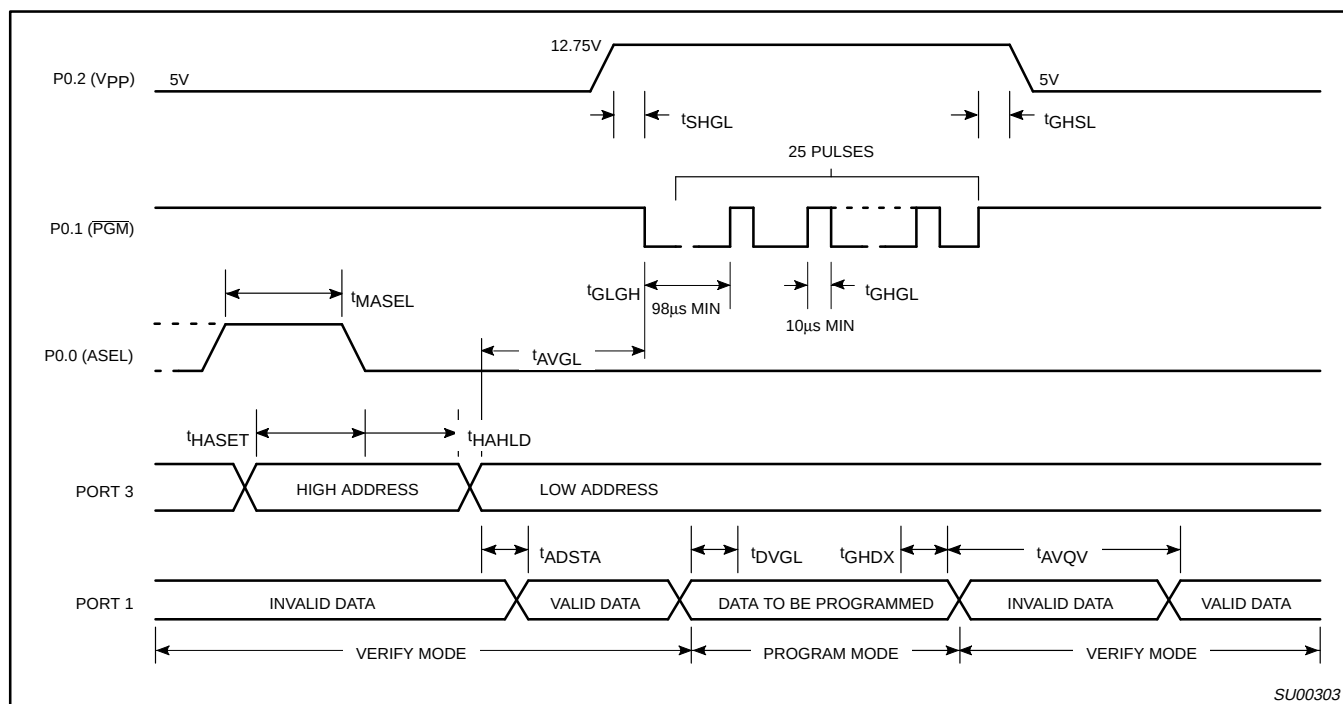
Figure 7. Program/Verify Cycle
