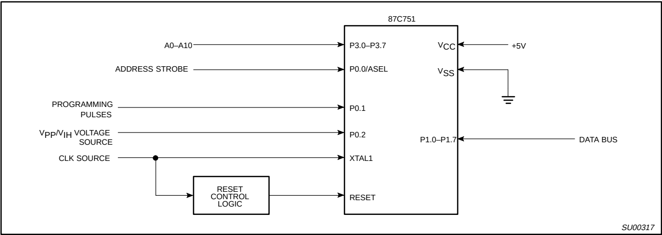
Figure 5. Programming Configuration
