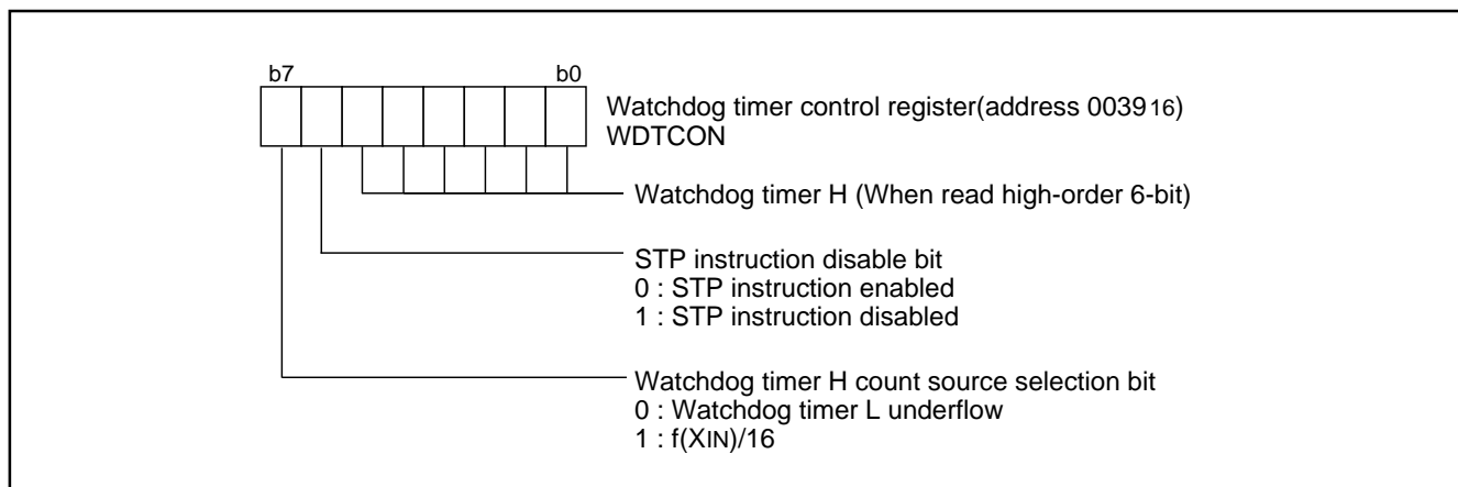
Fig. 35 Structure of watchdog timer control register
