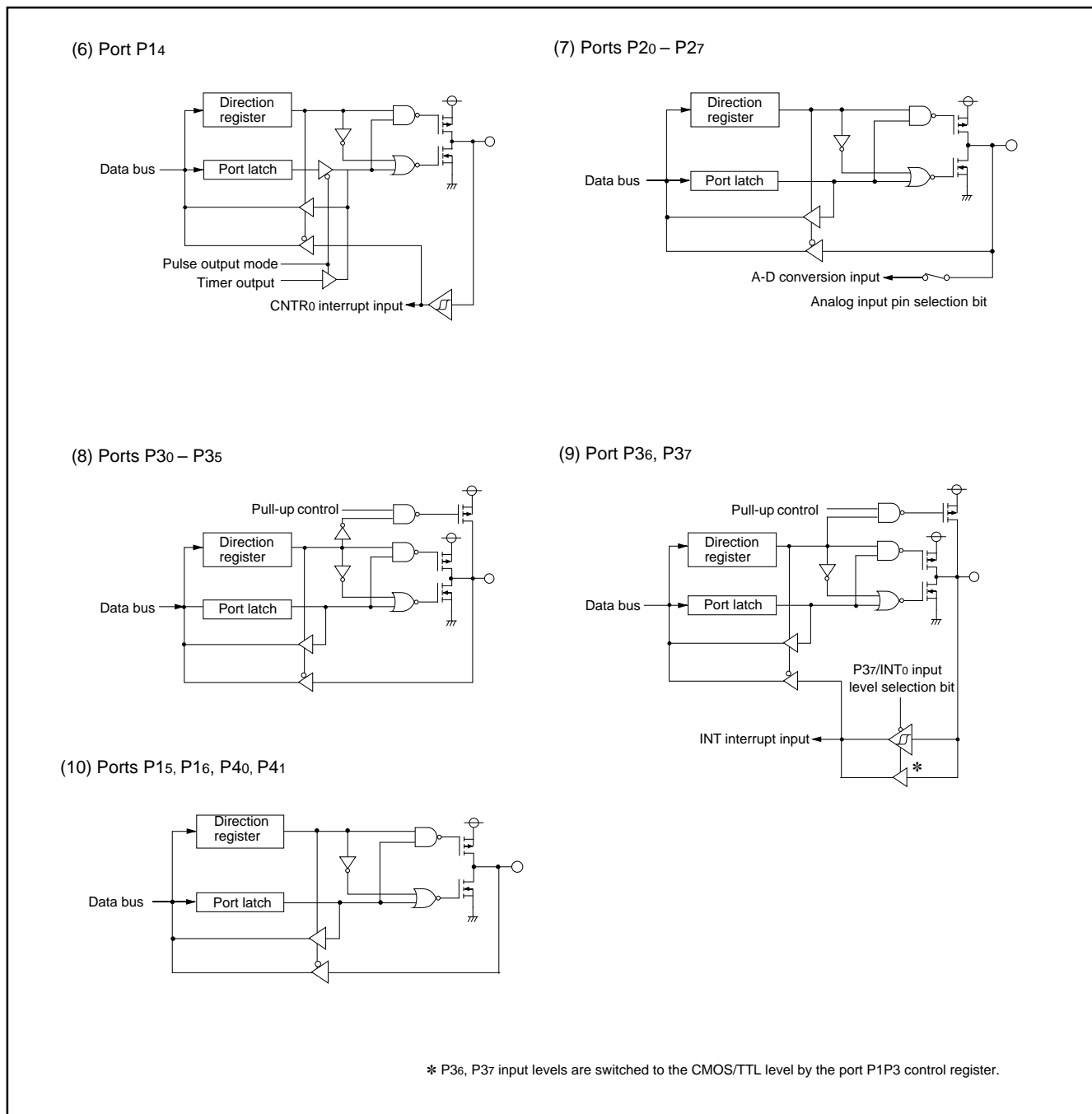
Fig. 11 Block diagram of ports (2)
