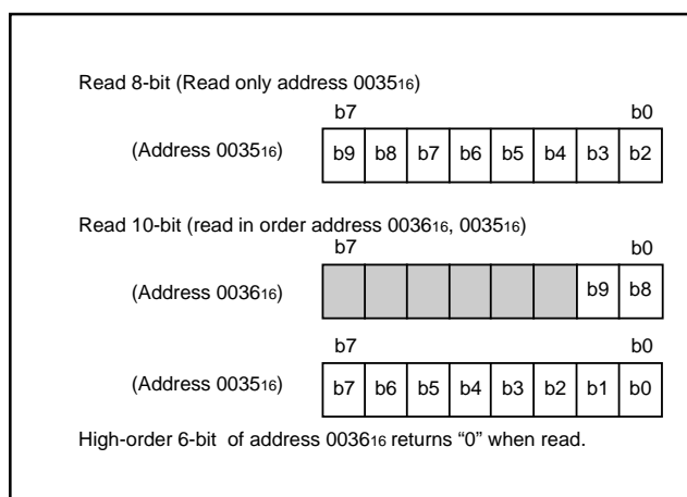
Fig. 32 Structure of A-D conversion register
