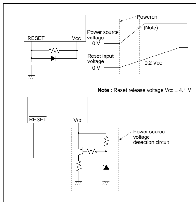
Fig. 36 Example of reset circuit
