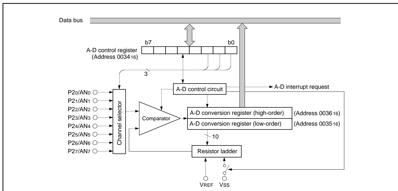
Fig. 33 Block diagram of A-D converter
