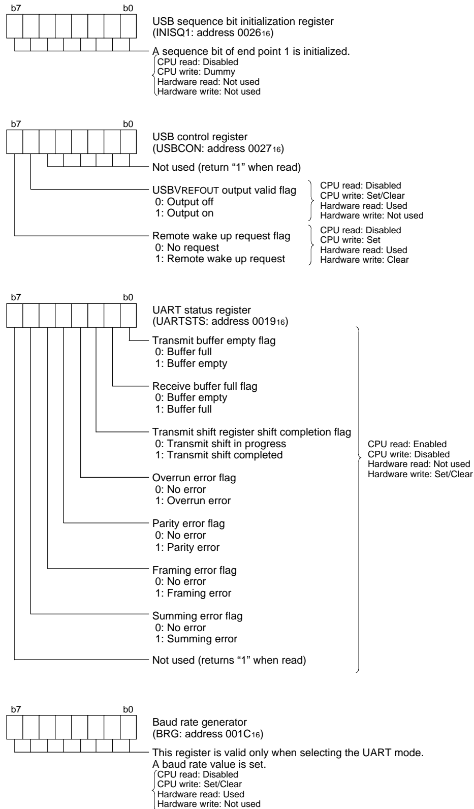
Fig. 26 Structure of serial I/O1-related registers (4)
