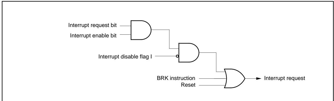
Fig. 12 Interrupt control
