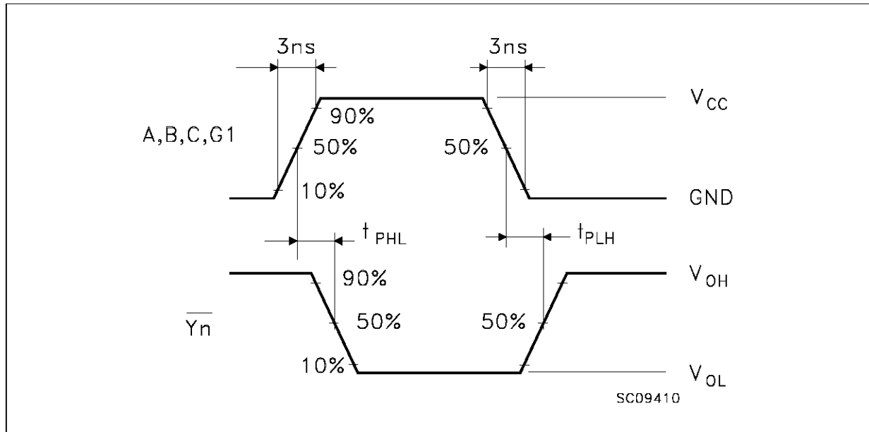
WAVEFORM 1: PROPAGATION DELAYS FOR INVERTING OUTPUTS ( f=1\text{MHz} ; duty cycle 50%)
