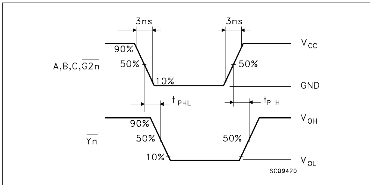
WAVEFORM 2: PROPAGATION DELAYS FOR NON-INVERTING OUTPUTS ( f=1\text{MHz} ; duty cycle 50%)
