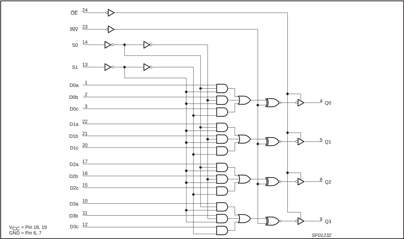
LOGIC DIAGRAM – 74F723A/74F723-1
