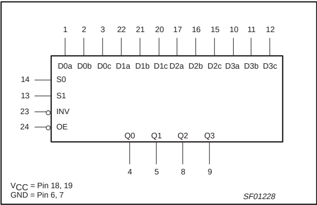
LOGIC SYMBOL – 74F723A/74F723-1
