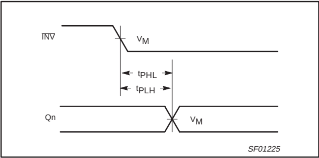
Waveform 3. Propagation Delay for \overline{INV} to Output
