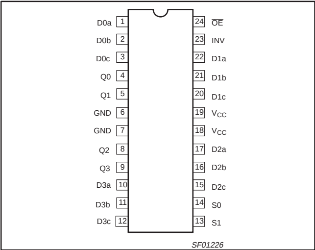
PIN CONFIGURATION – 74F723A/74F723-1
