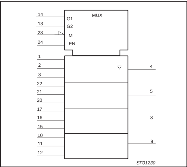
LOGIC SYMBOL (IEEE/IEC) – 74F723A/74F723-1
