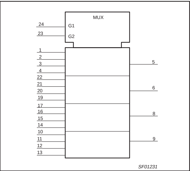
LOGIC SYMBOL (IEEE/IEC) – 74F725A/74F725-1
