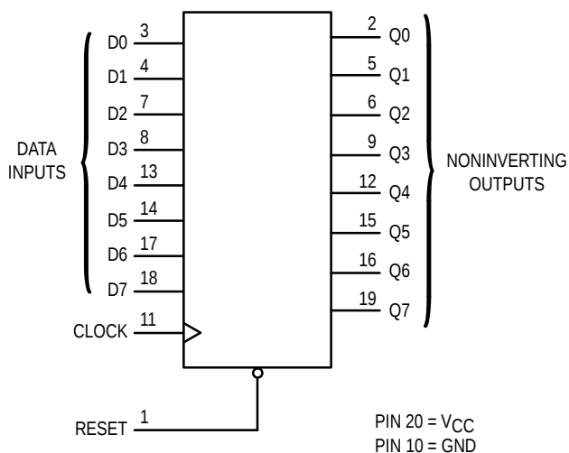
LOGIC DIAGRAM
