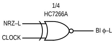
Figure 3. Biphas-Level Encoder (Manchester Encoder)
