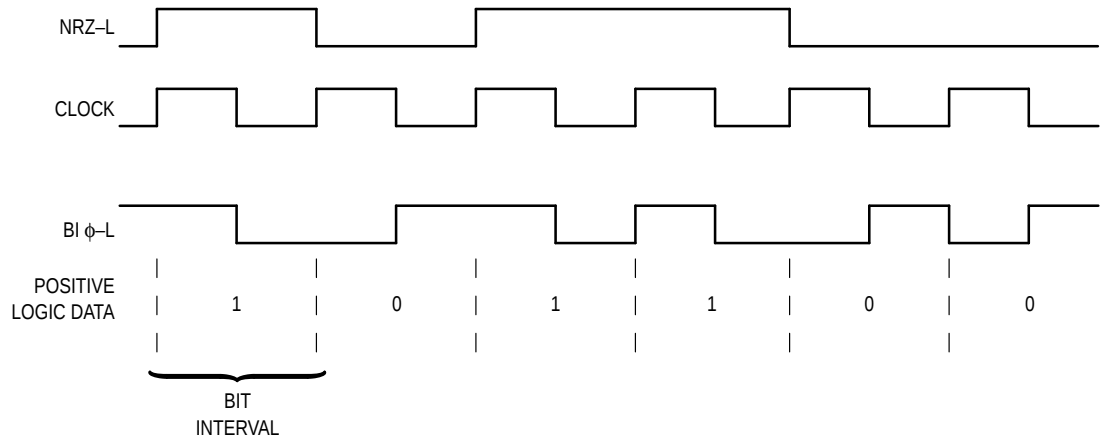
Figure 4. Timing Diagram
