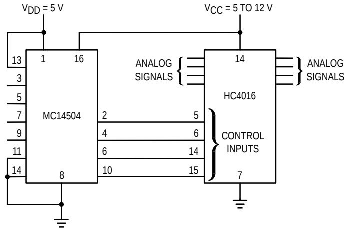
Figure 18. LSTTL/NMOS to HCMOS Interface
