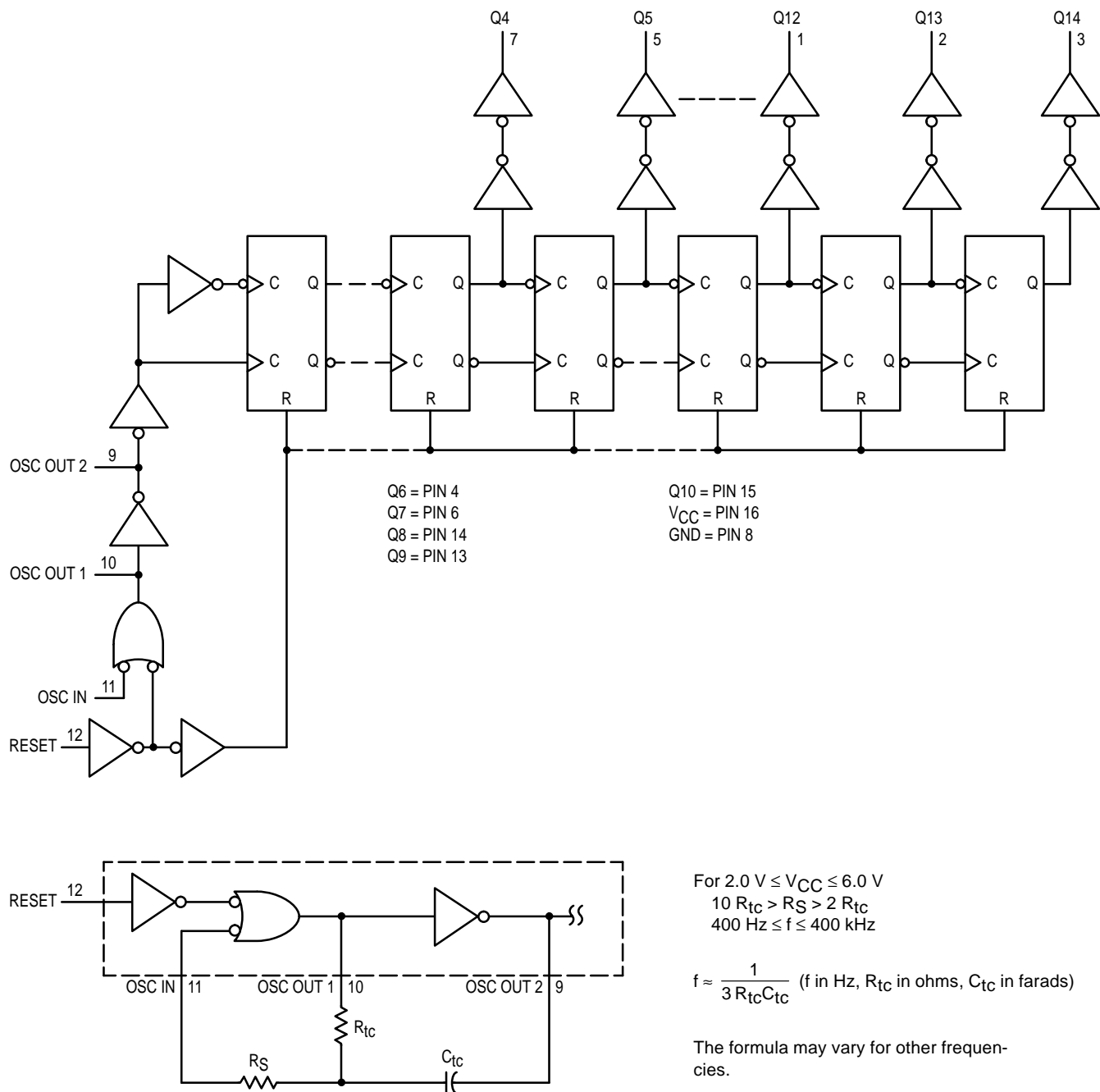
Figure 5. Oscillator Circuit Using RC Configuration
