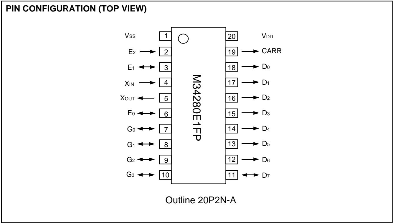
Fig. 26 Pin configuration of built-in PROM version
