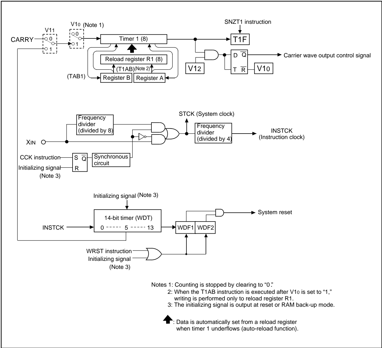
Fig. 13 Timers structure
