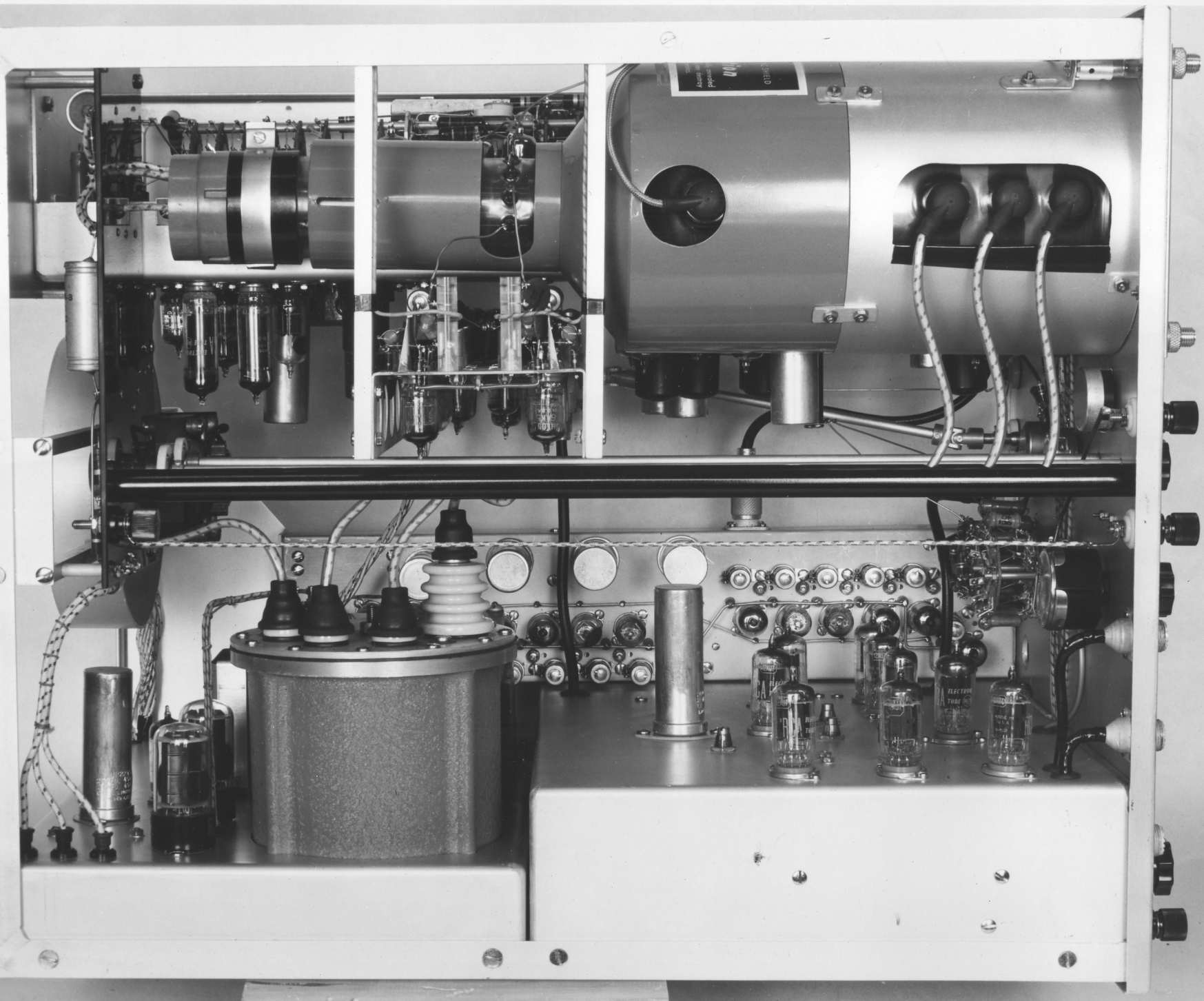
FIGURE 4 LEFT SIDE VIEW
