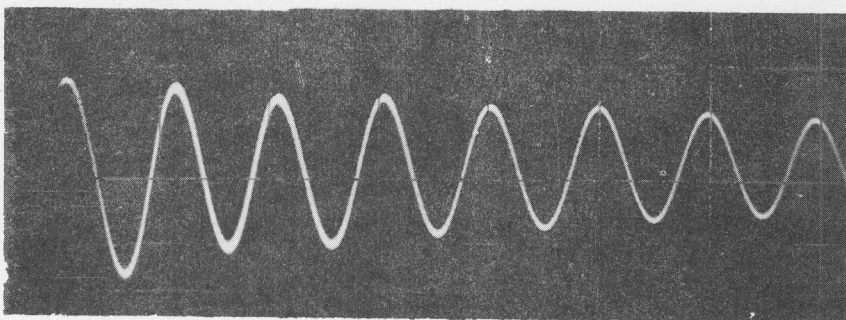
Fig. 26B -- 50 megacycle timing wave at sweep rate of 20 milliu sec/cm.
